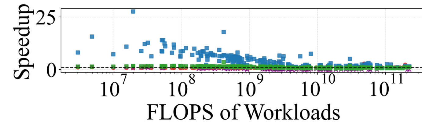
(h) Conv-BN-Add-ReLU on H100
