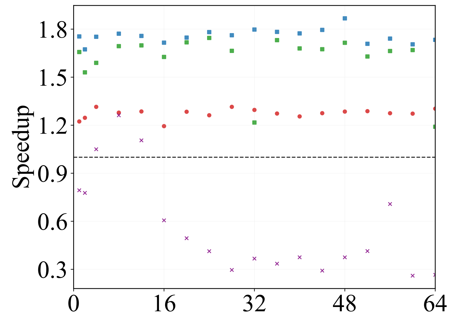
(h) AlexNet on H100
