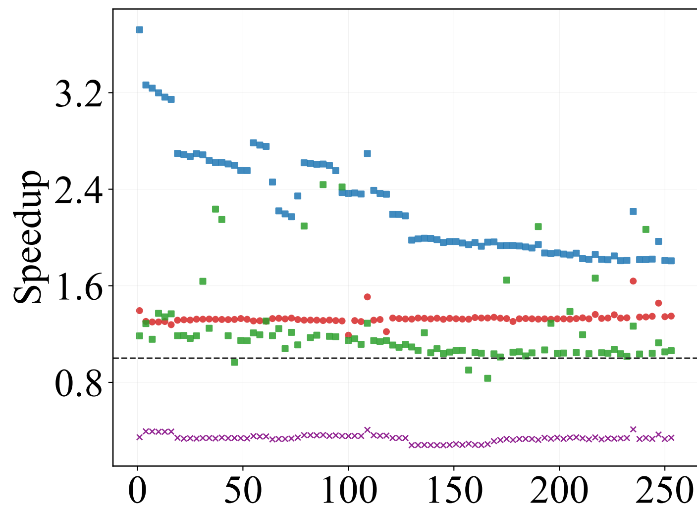
(b) BERT-base on A100
