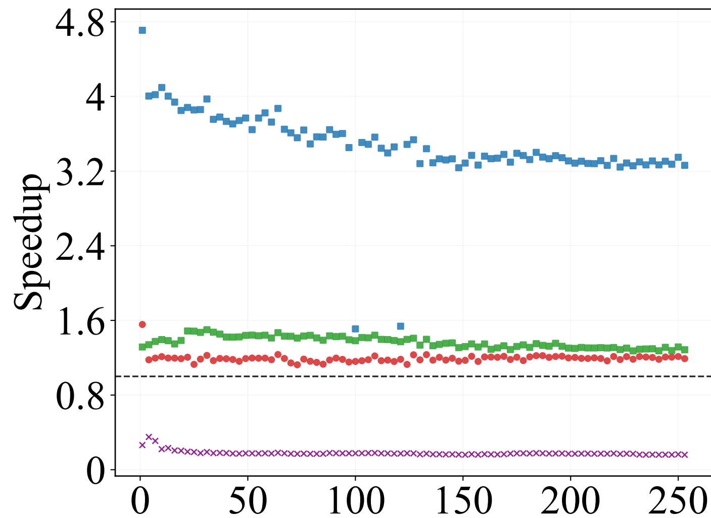
(f) BERT-base on H100
