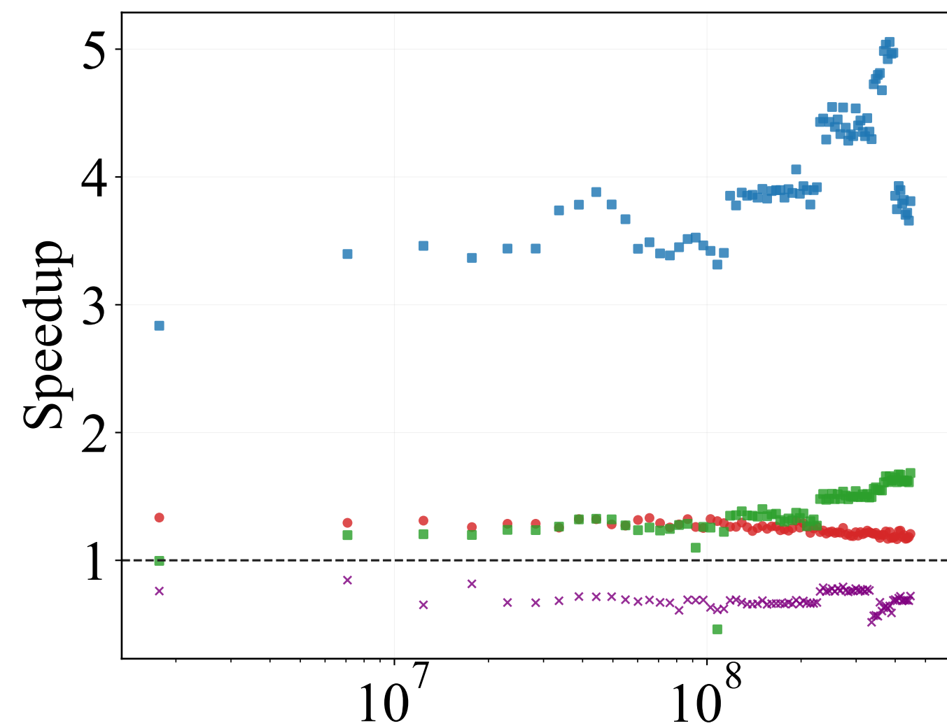
(e) GEMM-bias-activation on H100
