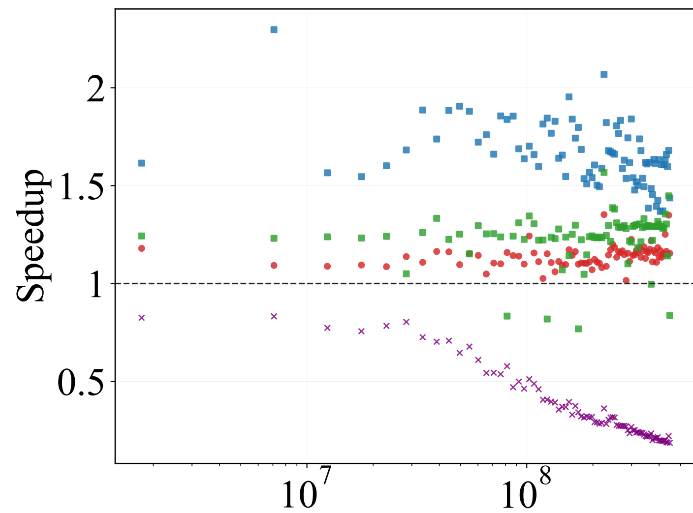
(b) GEMM-bias-layernorm on A100
