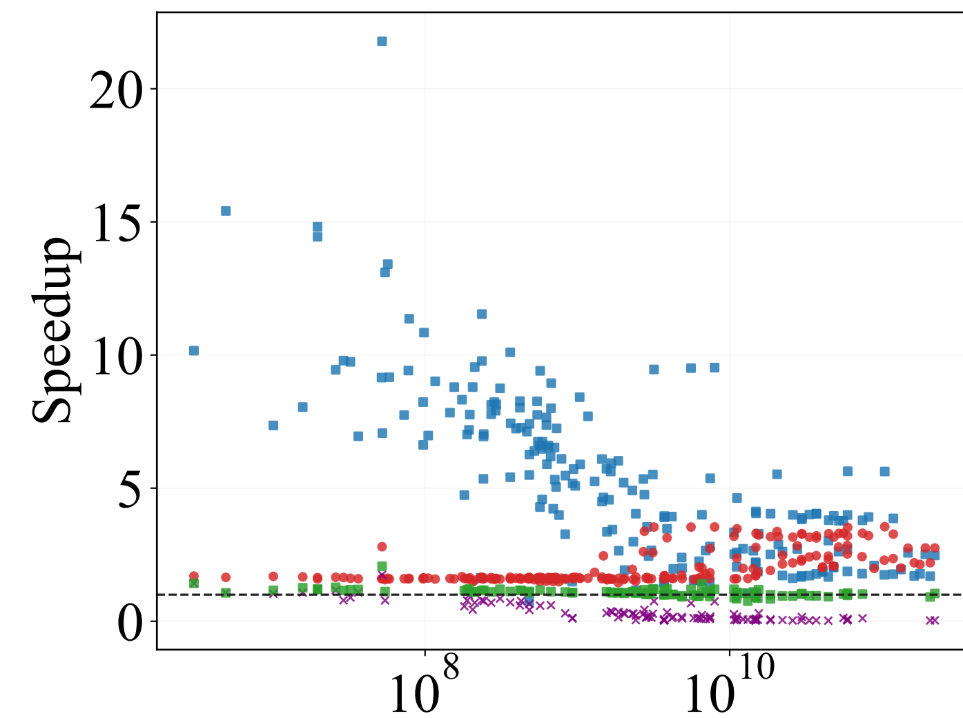
(h) Conv-BN-Add-ReLU on H100
