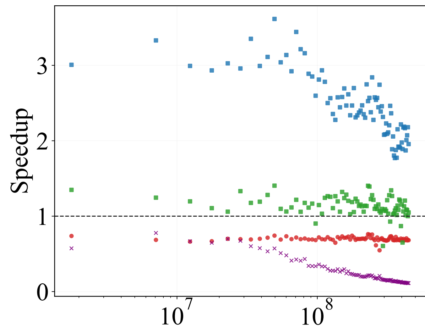
(a) GEMM-bias-activation on A100
