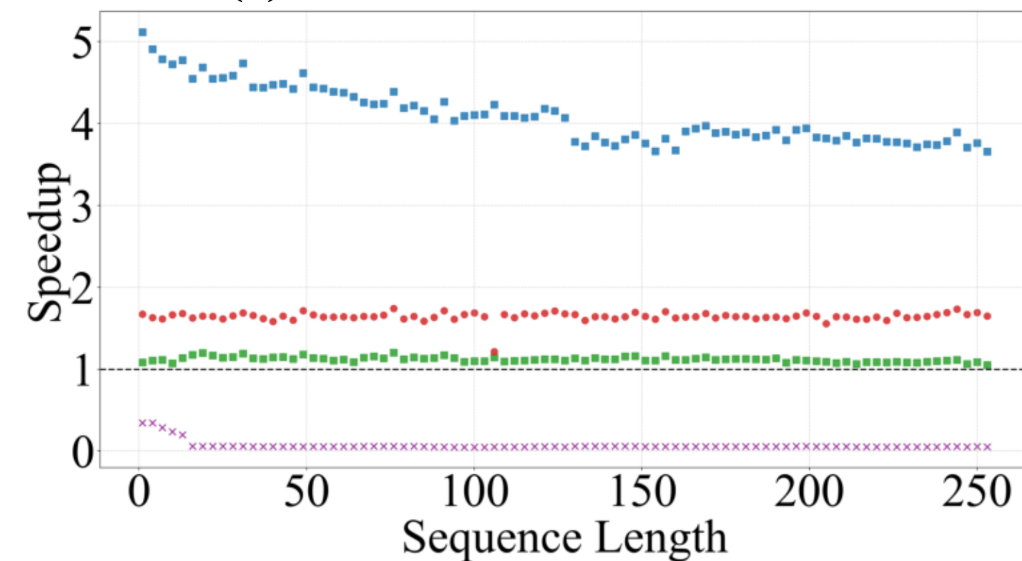
(c) LLaMA-base on H100
