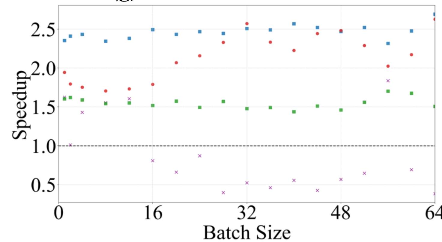
(g) ResNet101 on H100
