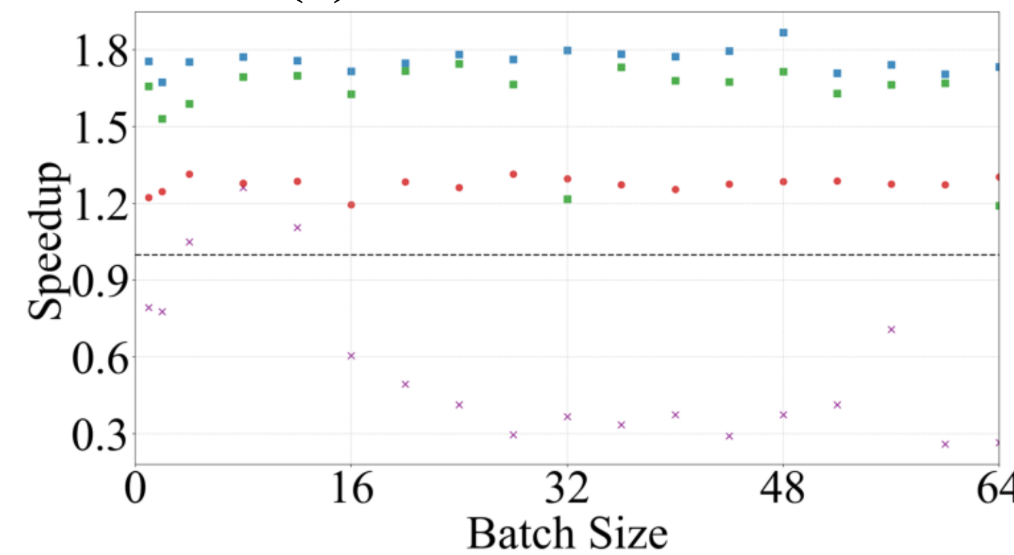
(h) AlexNet on H100
