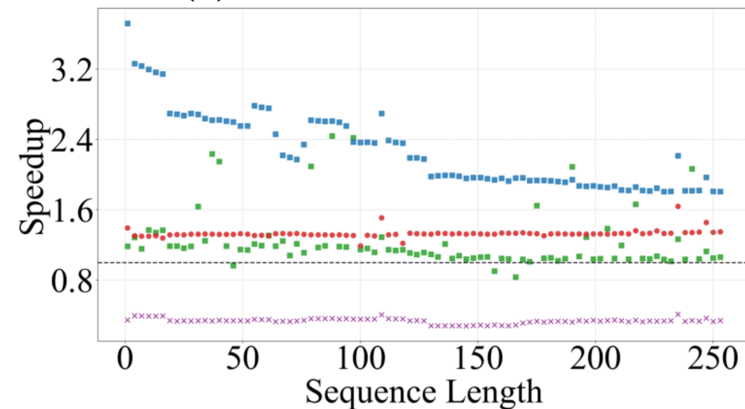
(b) BERT-base on A100
