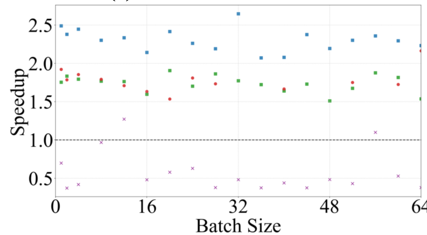
(e) ResNet101 on A100
