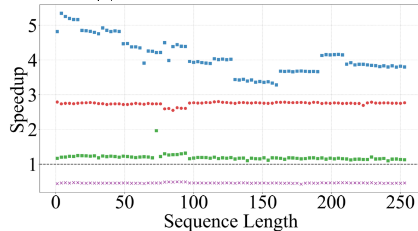
(a) LLaMA-base on A100
