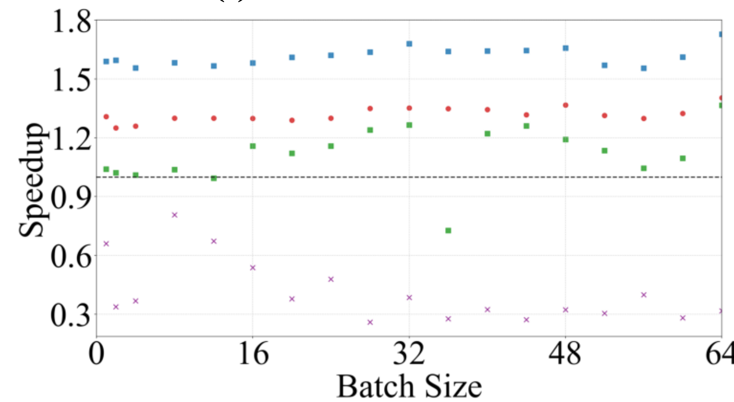
(f) AlexNet on A100
