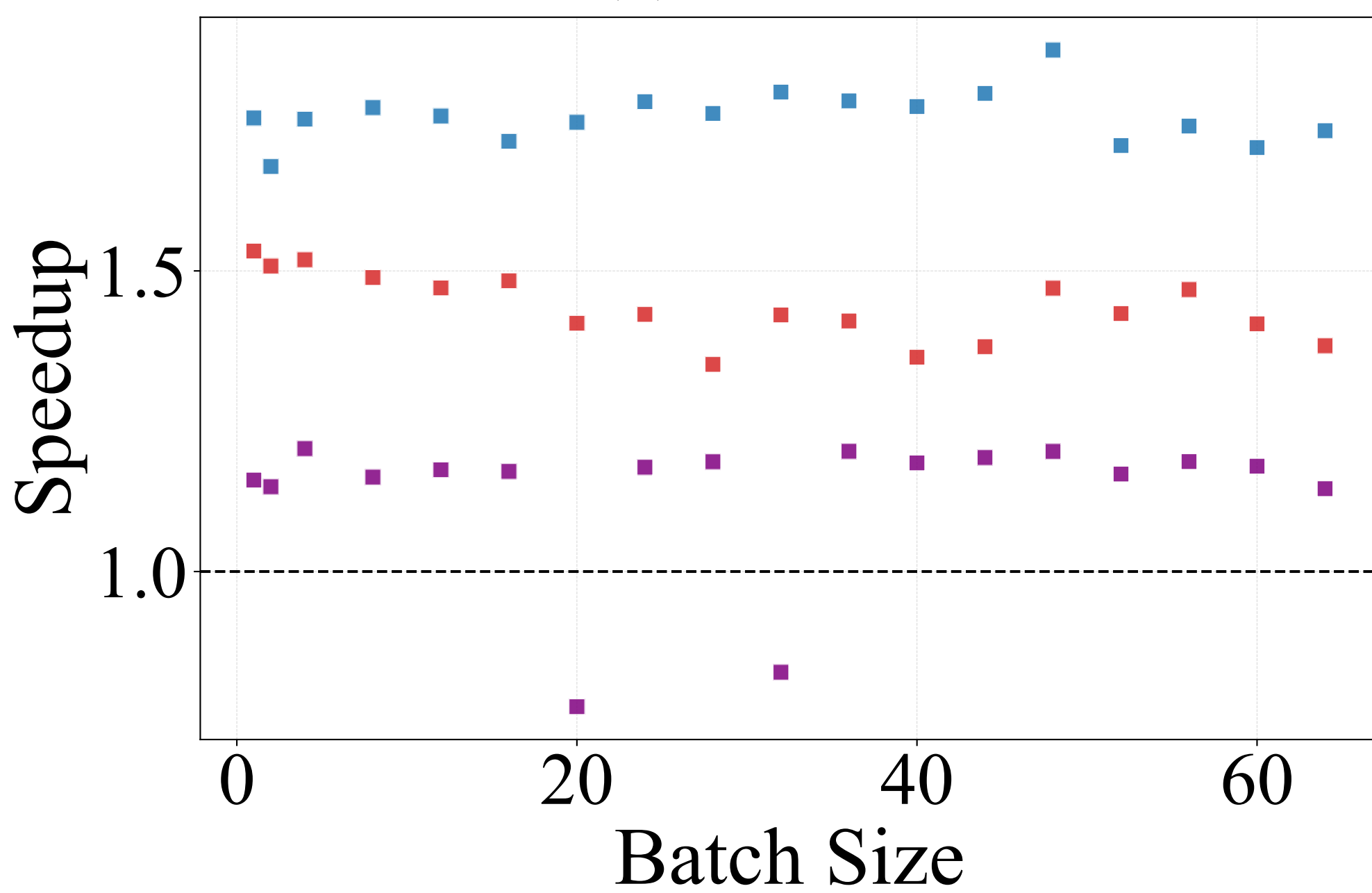
(c) AlexNet
