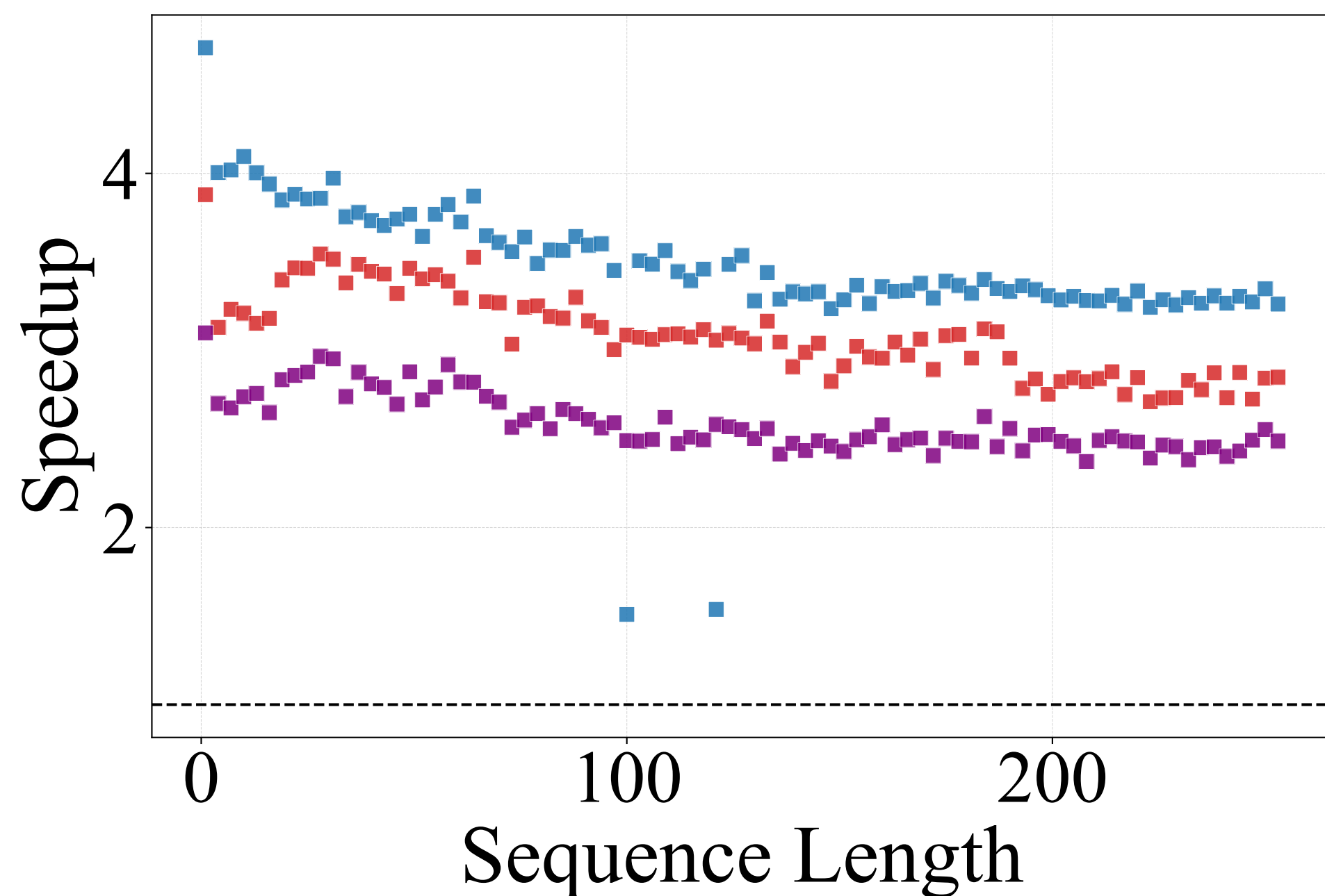
(c) AlexNet
