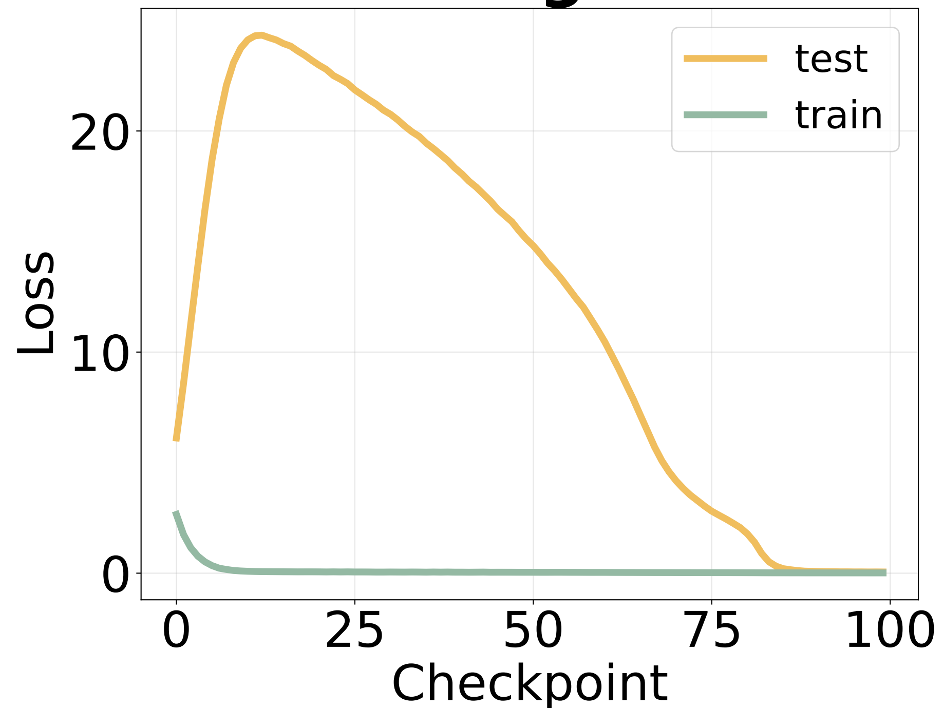
Feature Evolution
