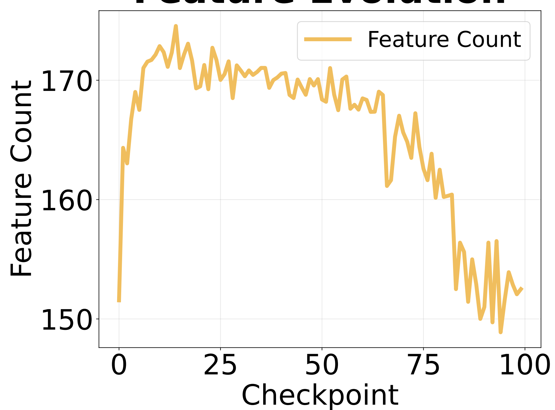
Feature Evolution
