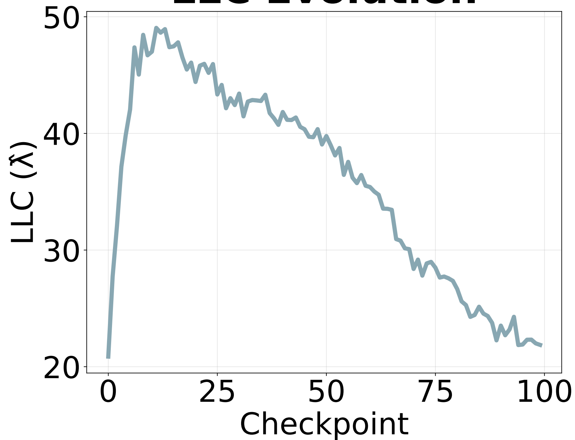
LLC Evolution
