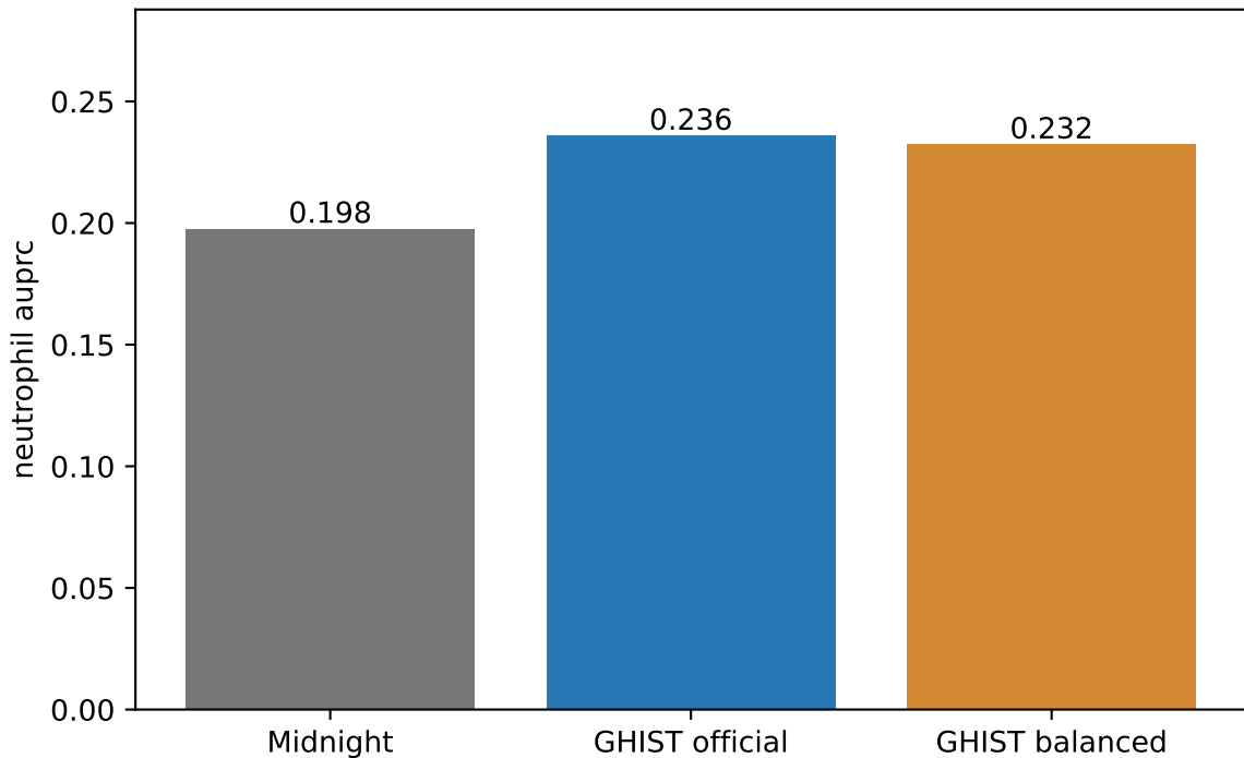
Neutrophil Auprc
