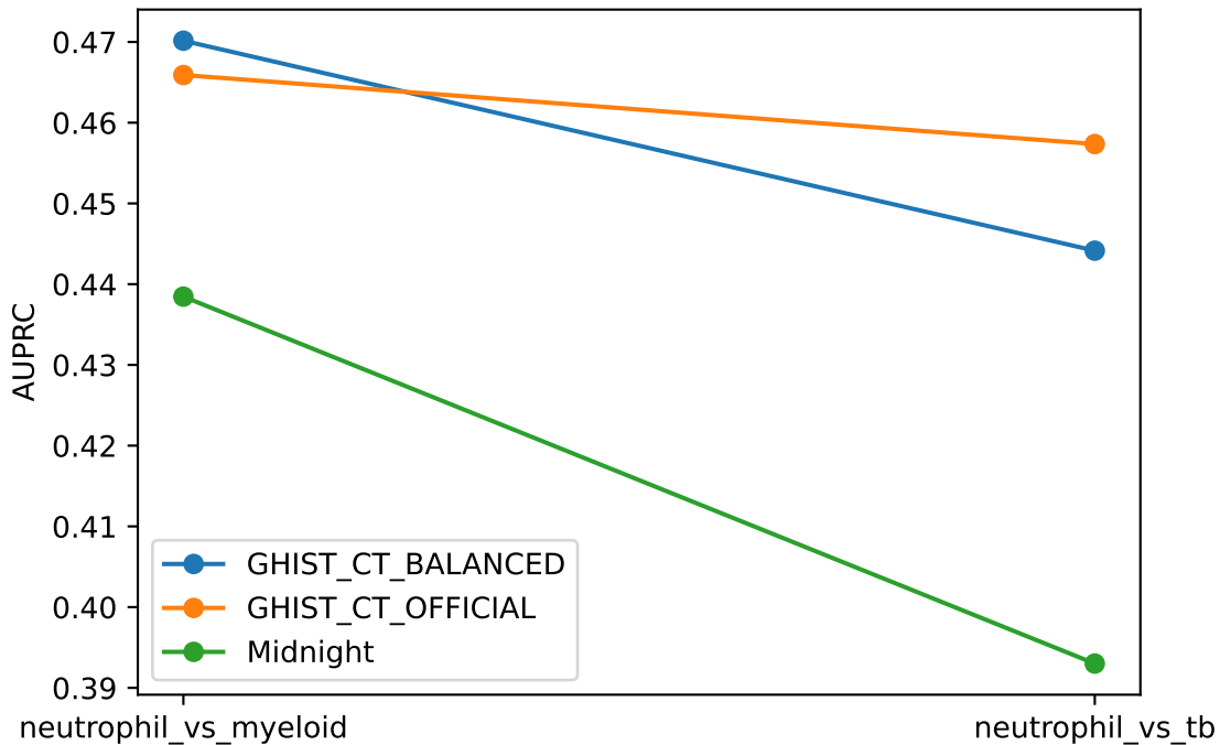
Training-only binary probes: AUPRC
