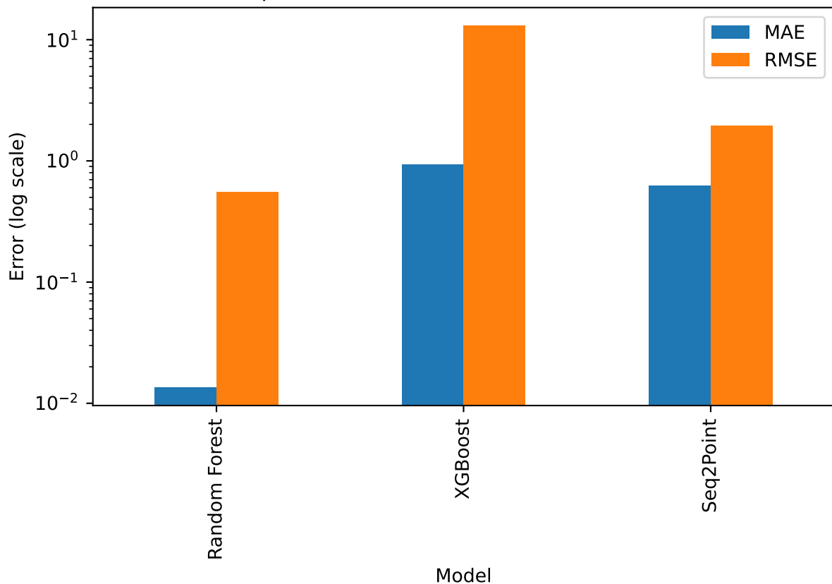
Comparison of NILM Models (MAE and RMSE)
