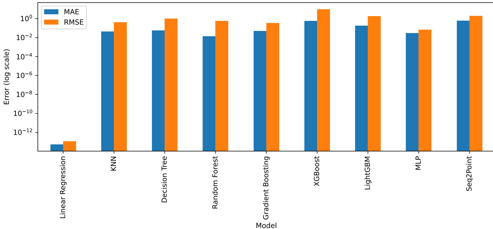
Comparison of NILM Models (MAE and RMSE)
