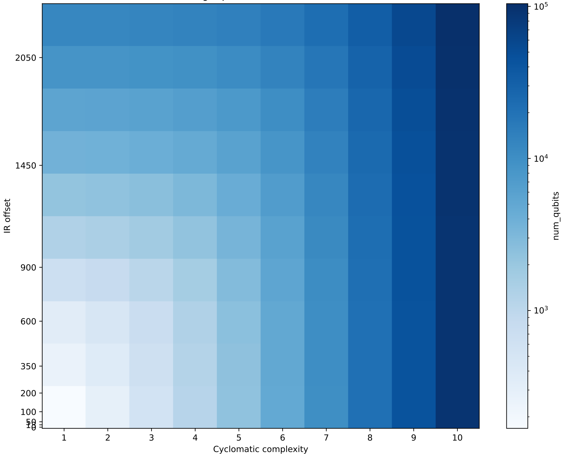
Average qubits vs CC and IR offset
