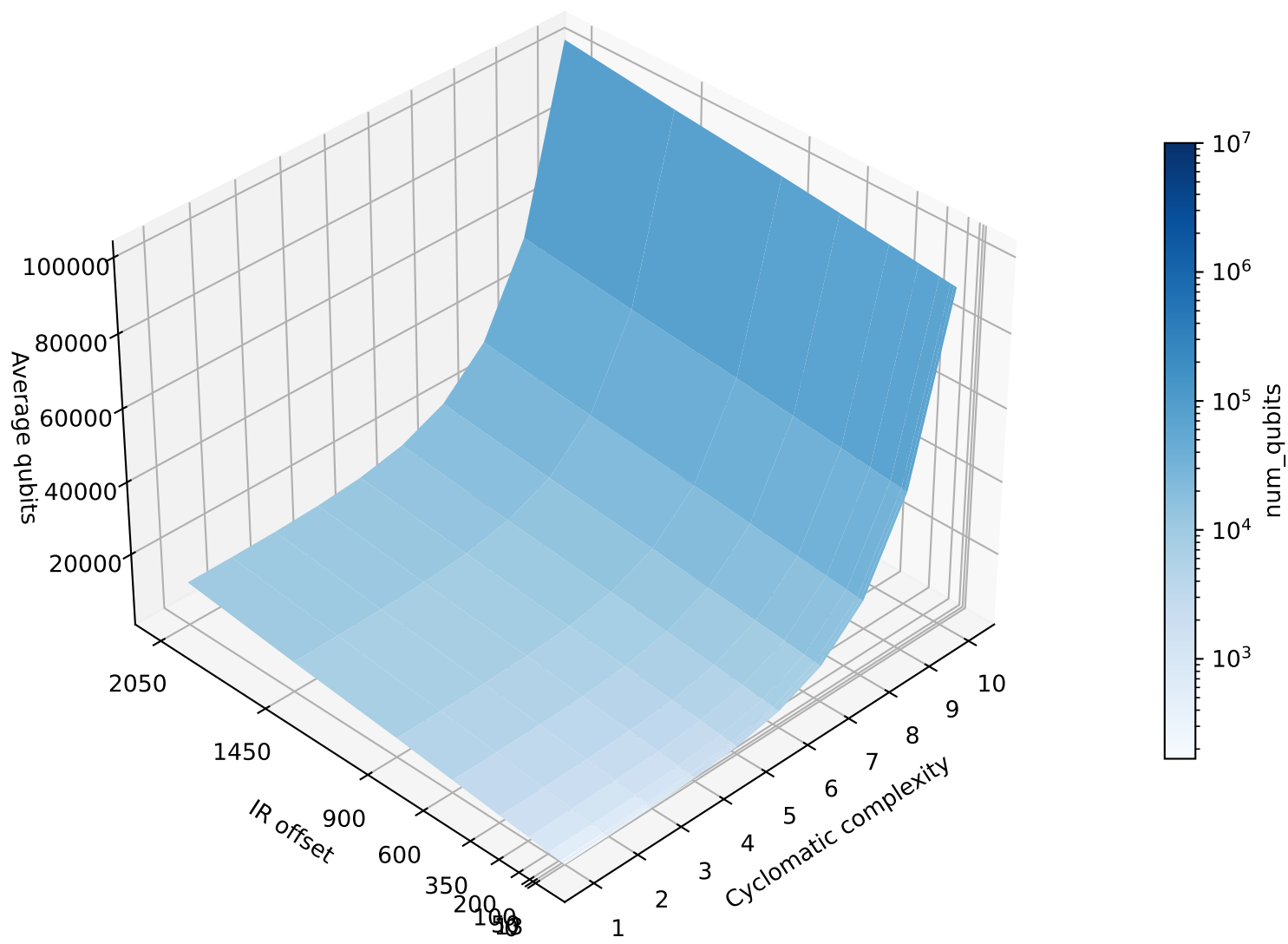
Average qubits vs CC and IR offset (surface)
