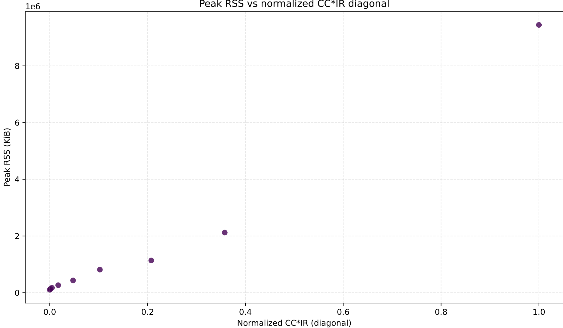
Peak RSS vs normalized CC*IR diagonal
