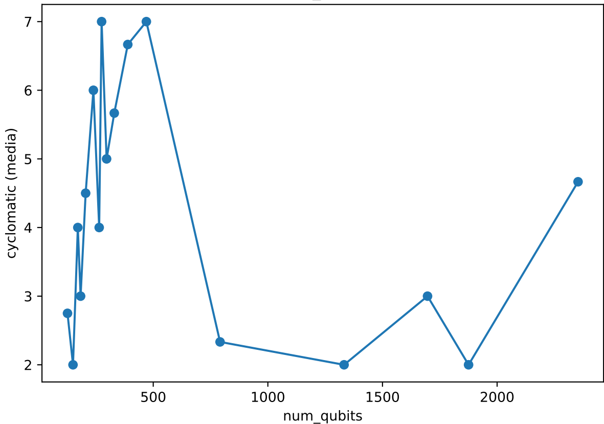
cyclomatic vs num_qubits (media su lr)
