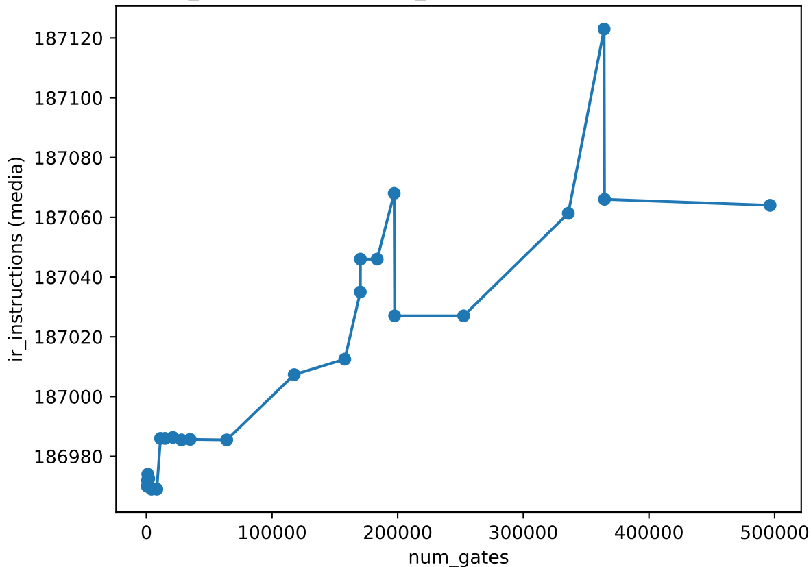
ir_instructions vs num_gates (media su ciclomatic)
