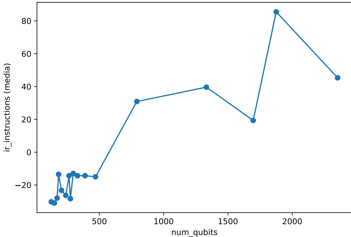
ir_instructions vs num_qubits (media su ciclomatic)
