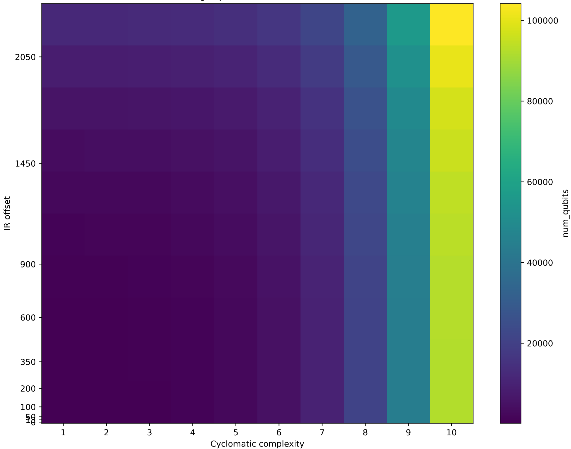
Average qubits vs CC and IR offset
