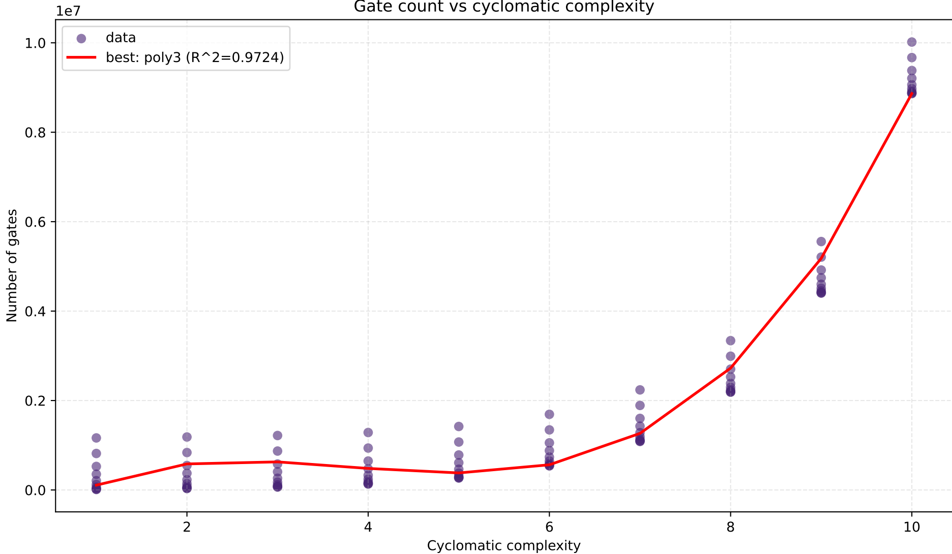
Gate count vs cyclomatic complexity
