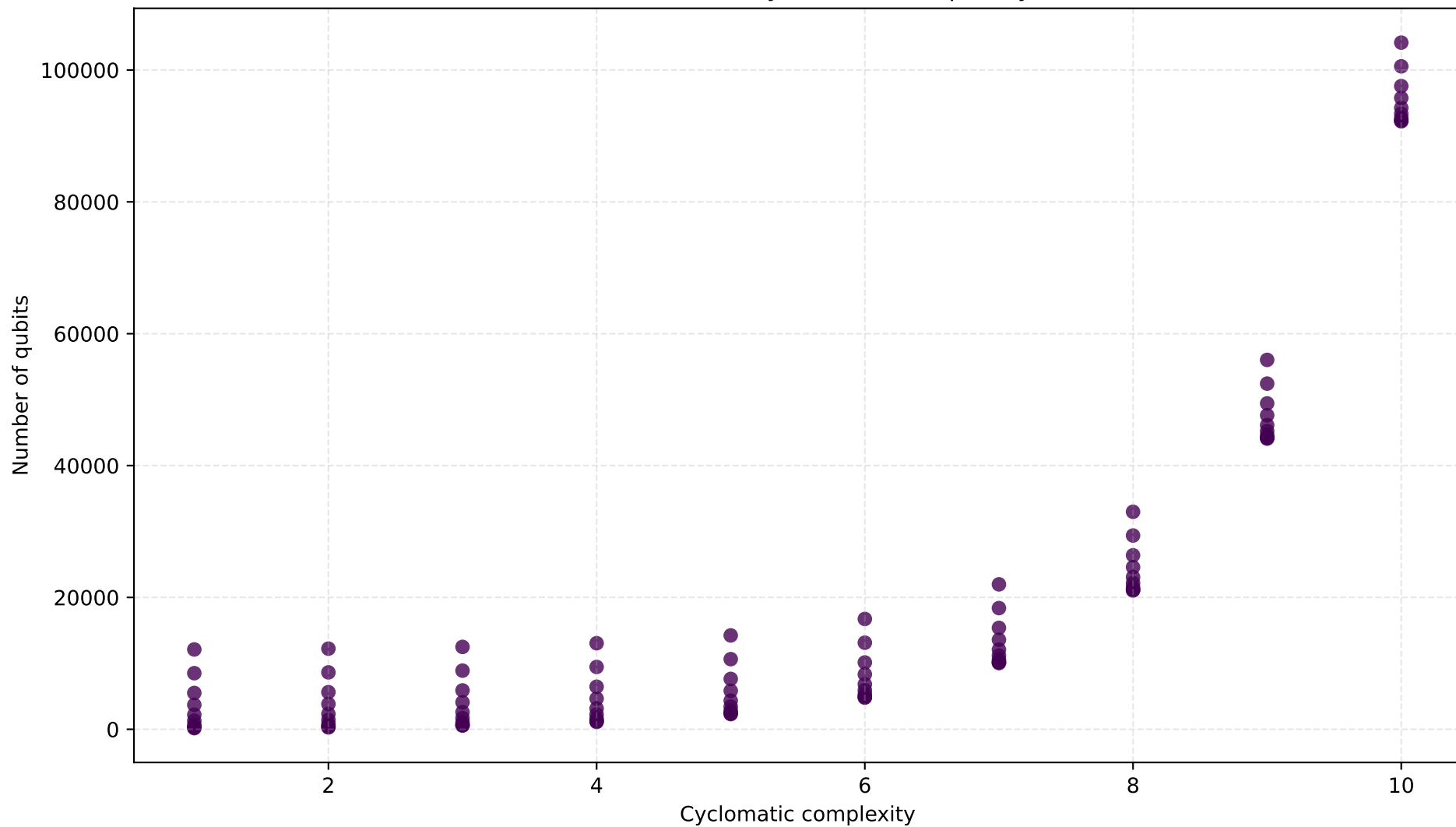
Qubit count vs cyclomatic complexity
