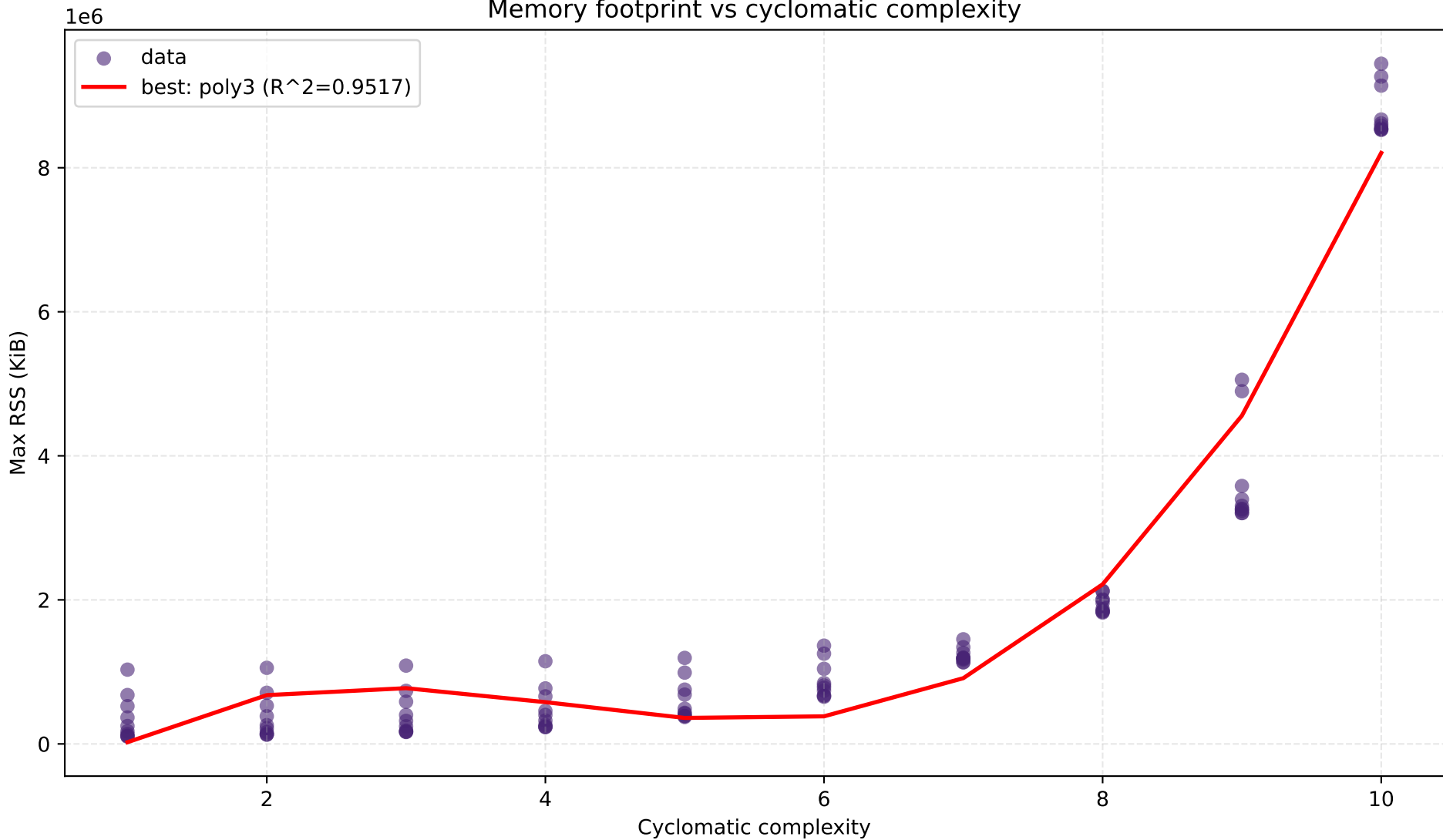
Memory footprint vs cyclomatic complexity
