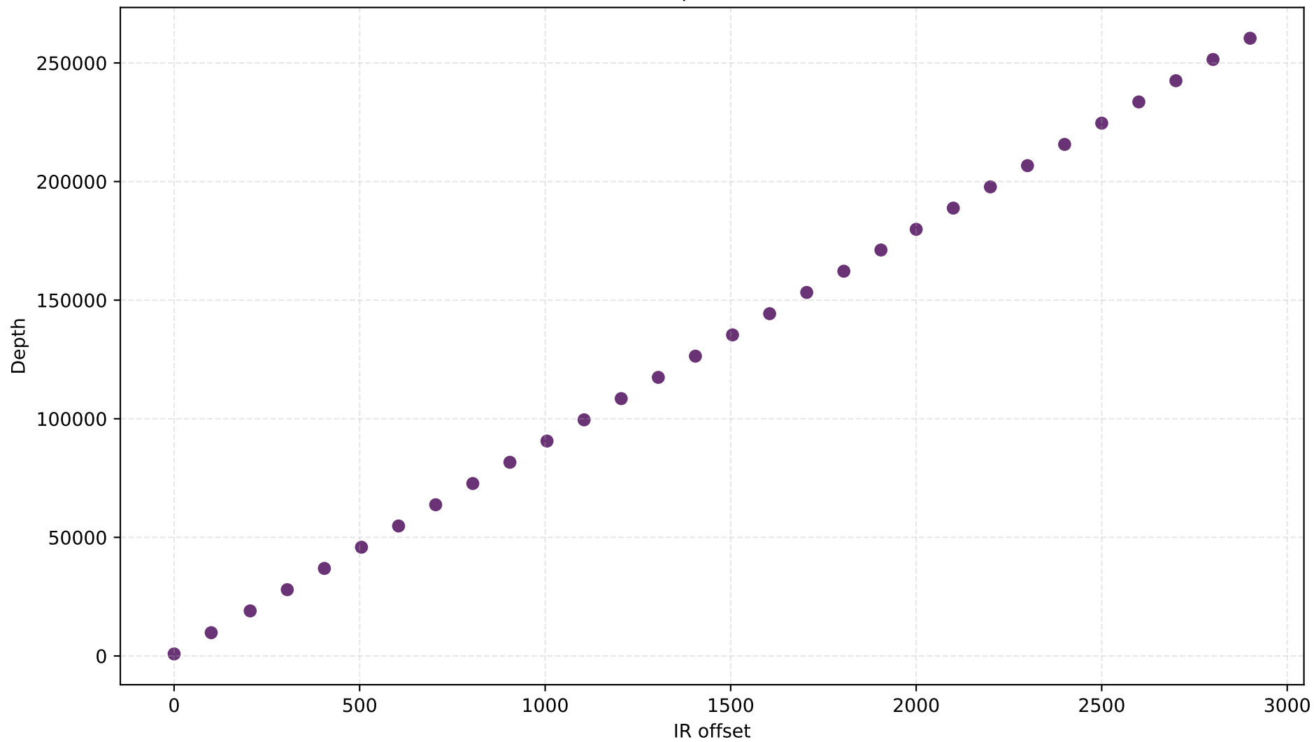
Circuit depth vs IR offset
