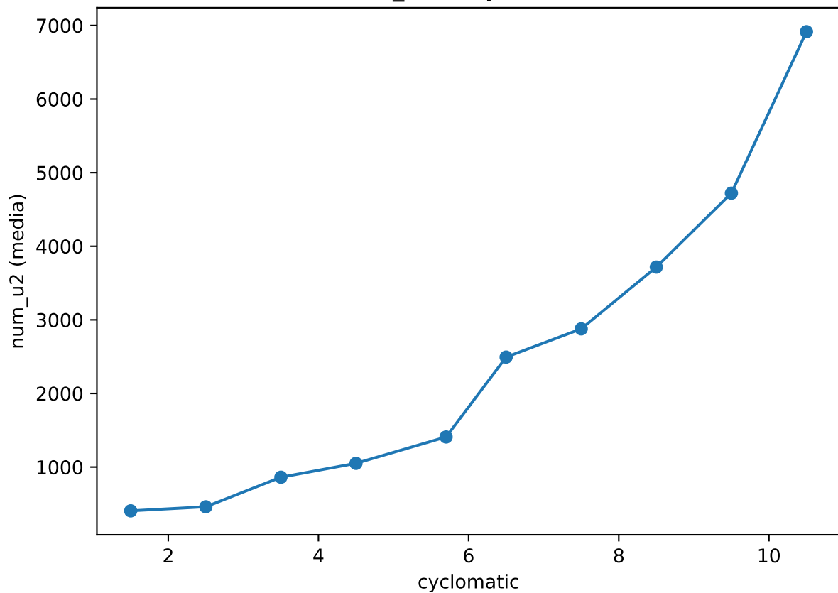
num_u2 vs cyclomatic
