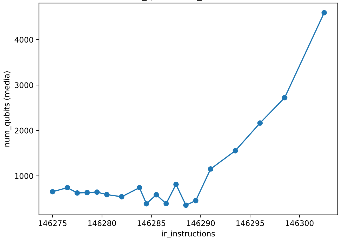
num_qubits vs ir_instructions
