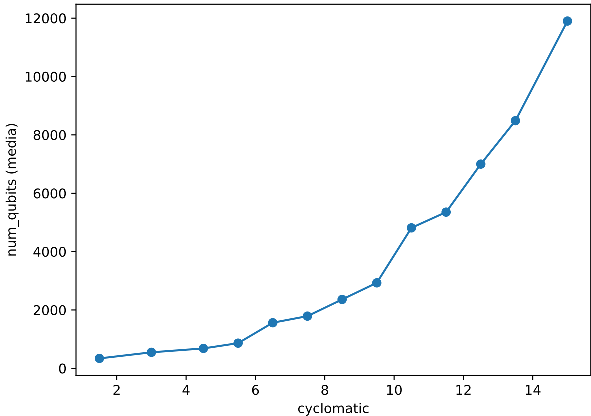
num_qubits vs cyclomatic
