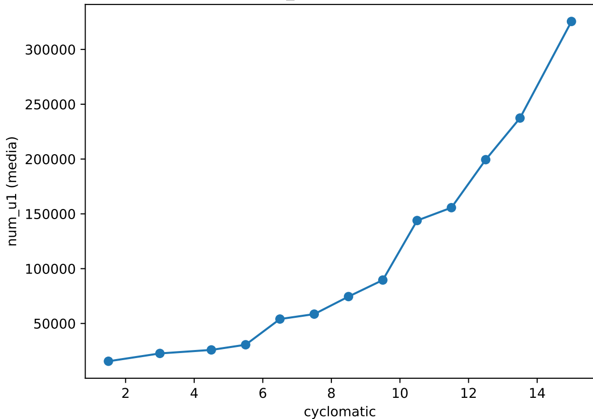
num_u1 vs cyclomatic
