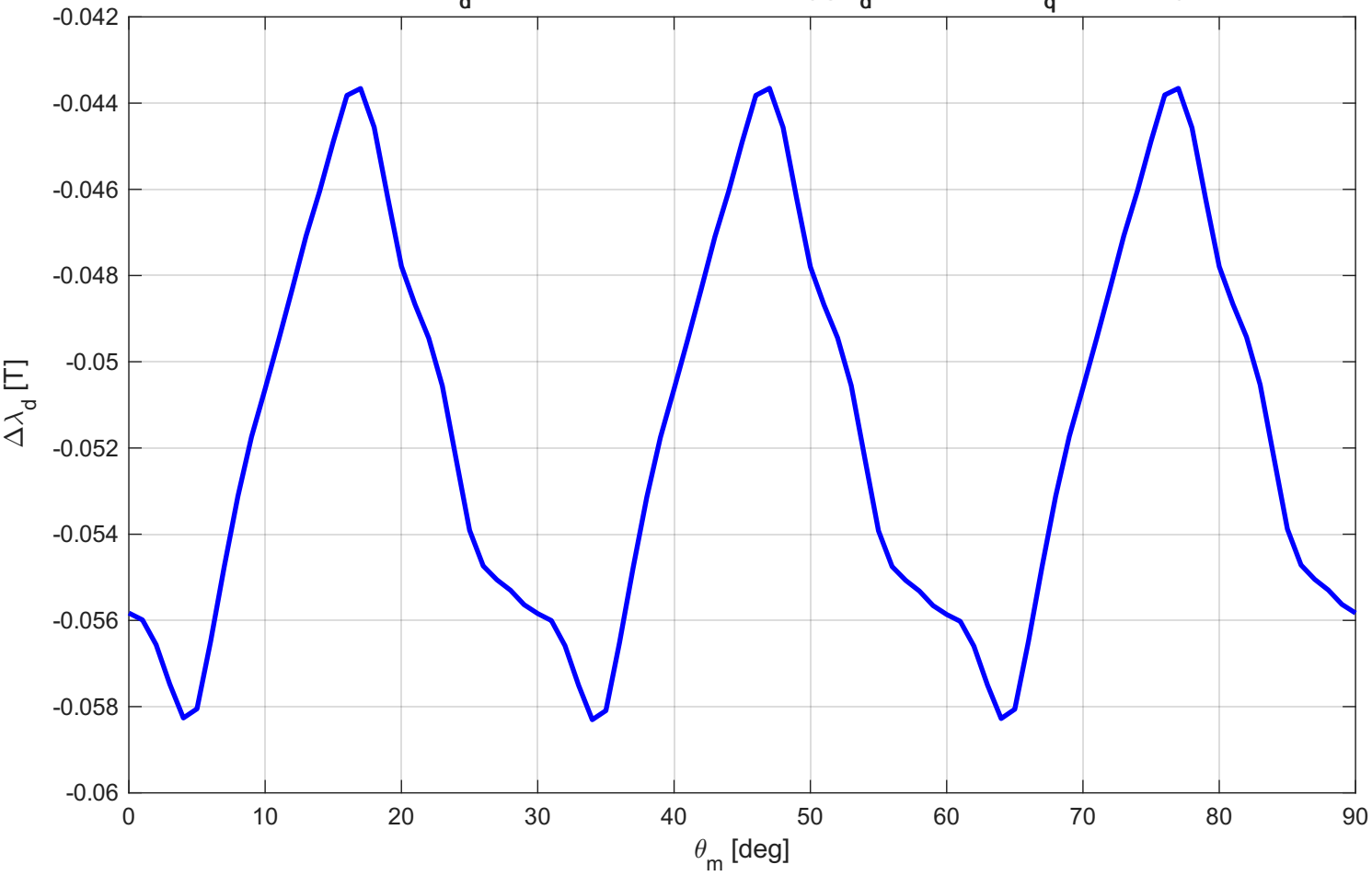
Differenza \lambda_d : MTPA vs Correnti Nulle (@ i_d = -2.755 A, i_q = 3.17 A)
