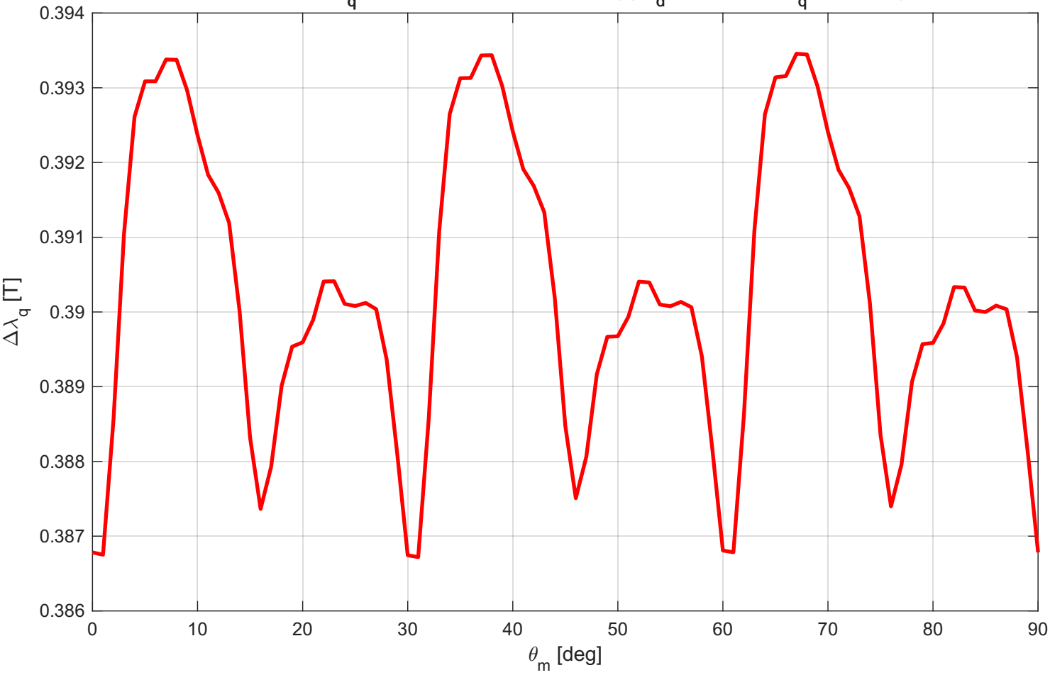
Differenza \lambda_q : MTPA vs Correnti Nulle (@ i_d = -2.755 A, i_q = 3.17 A)
