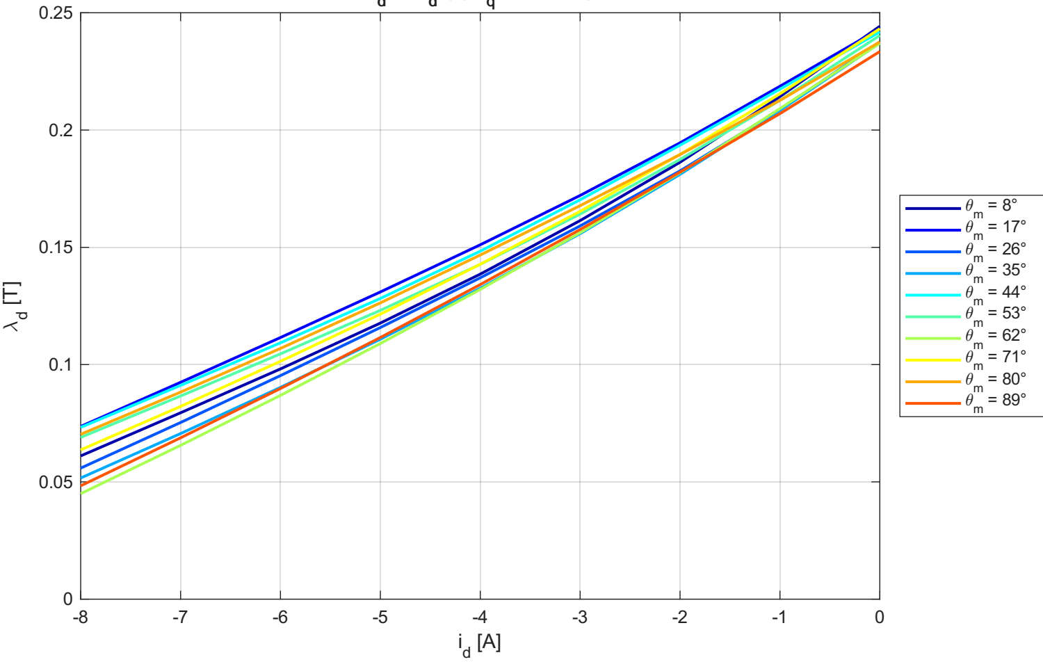
\lambda_d vs i_d (@ i_q = 3.17 A)
