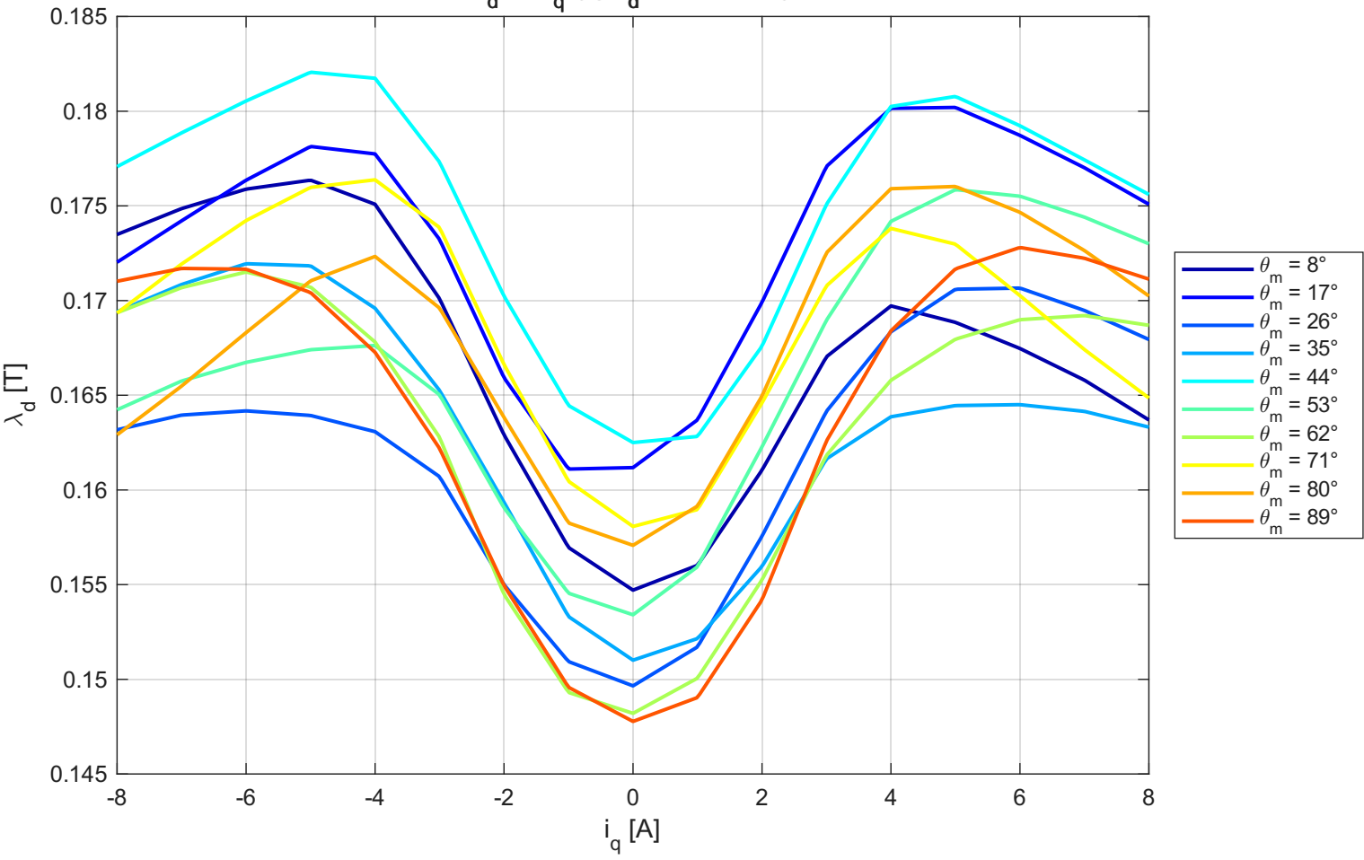
\lambda_d vs i_q (@ i_d = -2.755 A)
