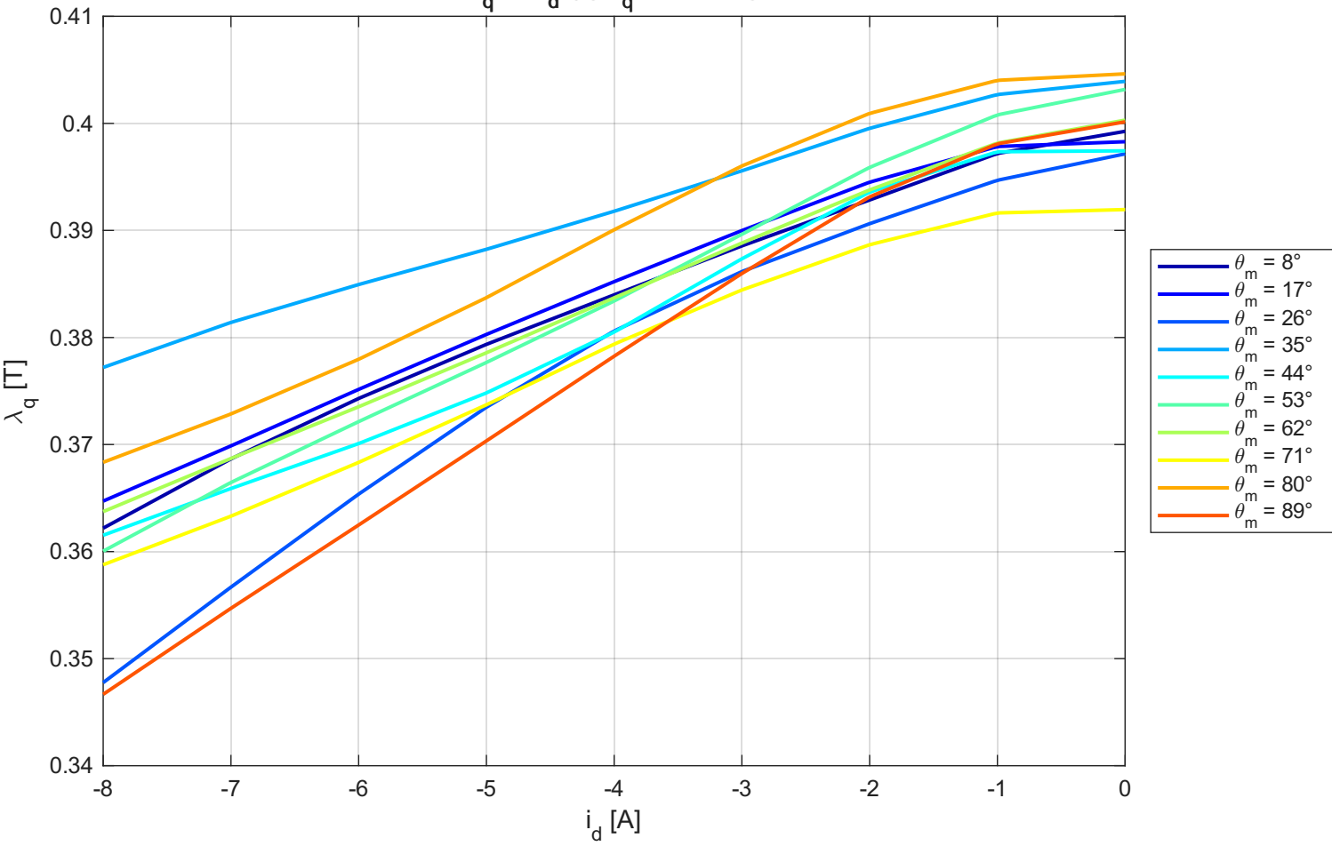
\lambda_q vs i_d (@ i_q = 3.17 A)
