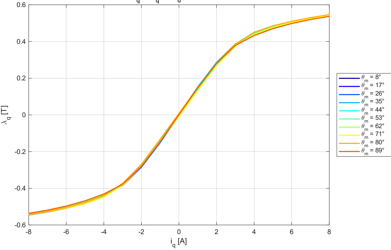
\lambda_q vs i_q (@ i_d = -2.755 A)
