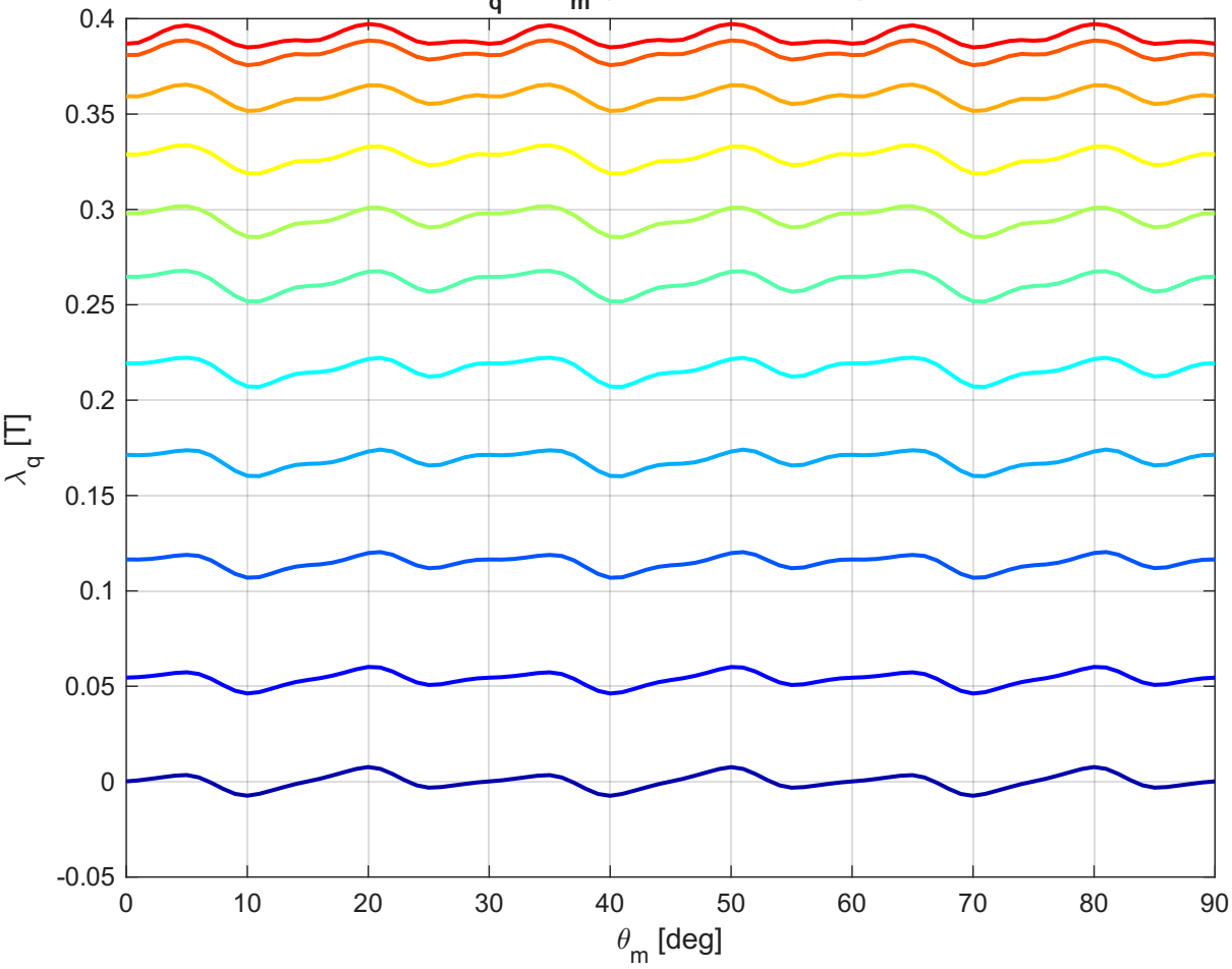
\lambda_q vs \theta_m (Traiettorie MTPA)
