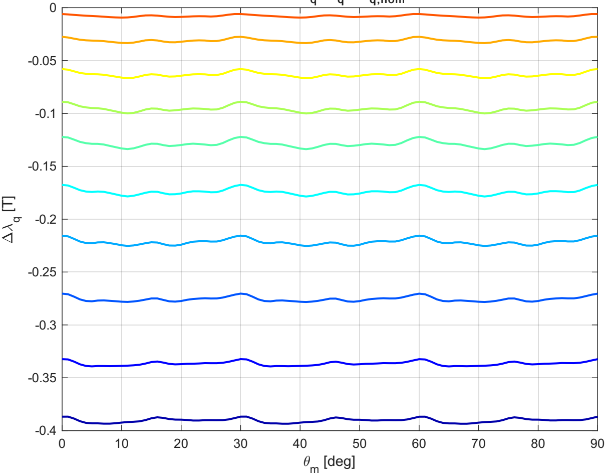
Differenza Assoluta \lambda_q ( \lambda_q - \lambda_{q,nom} ) lungo MTPA
