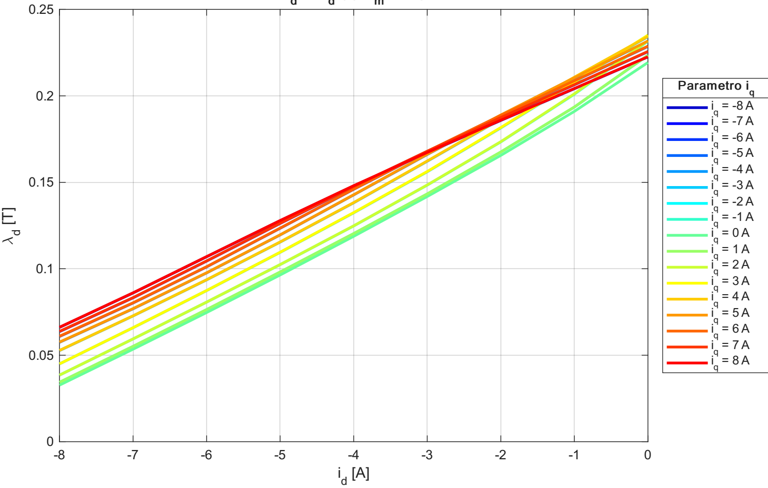
\lambda_d vs i_d (@ \theta_m = 0^\circ )
