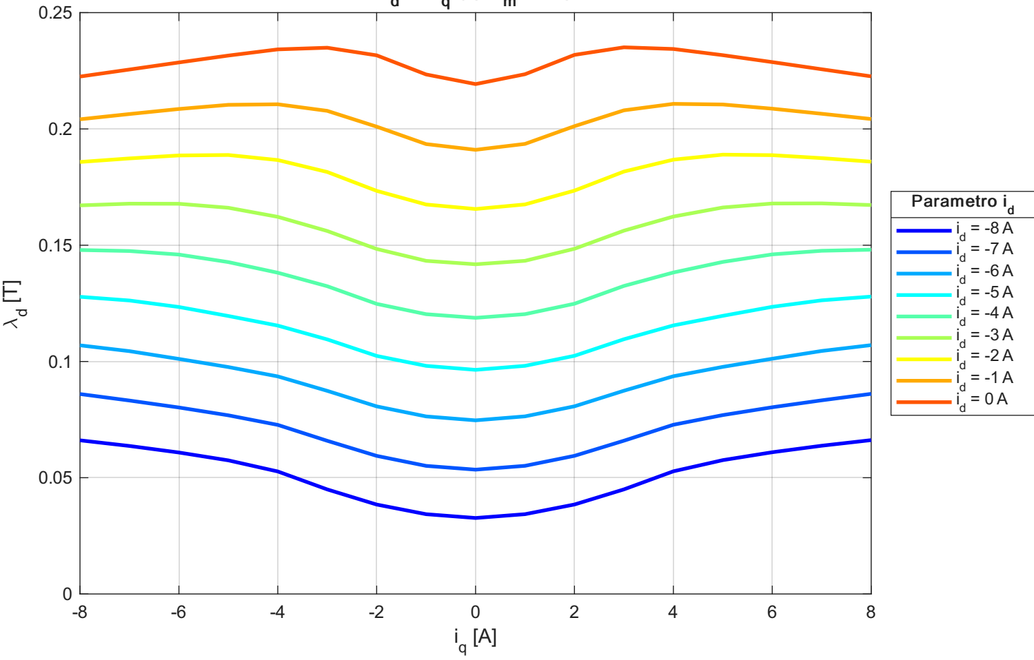
\lambda_d vs i_q (@ \theta_m = 0^\circ )
