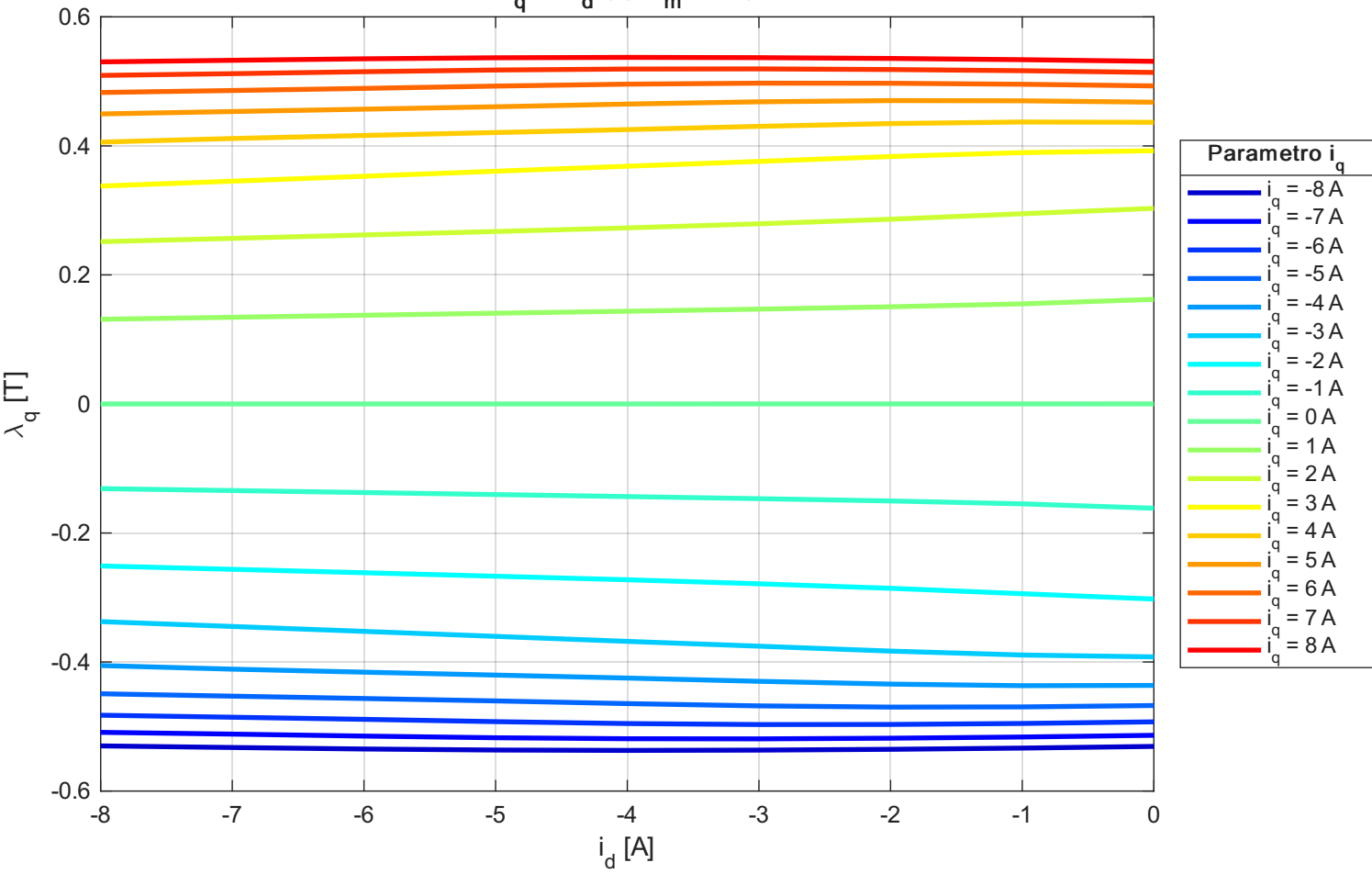
\lambda_q vs i_d (@ \theta_m = 0^\circ )
