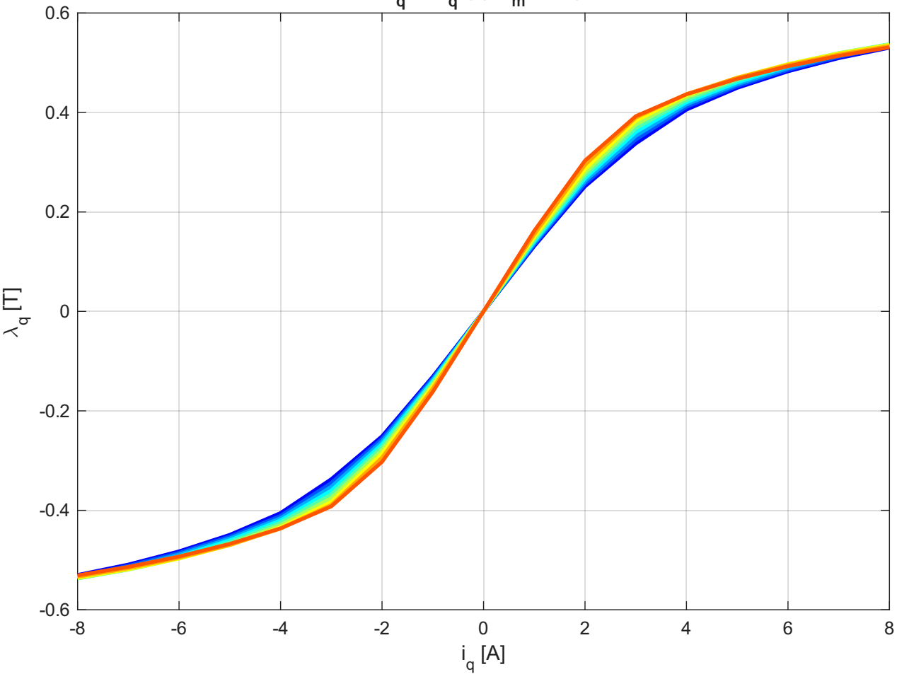
\lambda_q vs i_q (@ \theta_m = 0^\circ )
