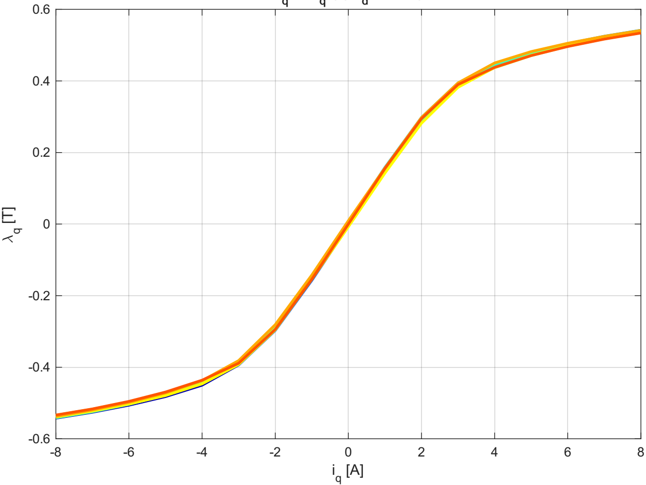
\lambda_q vs i_q (@ i_d = -1 A)
