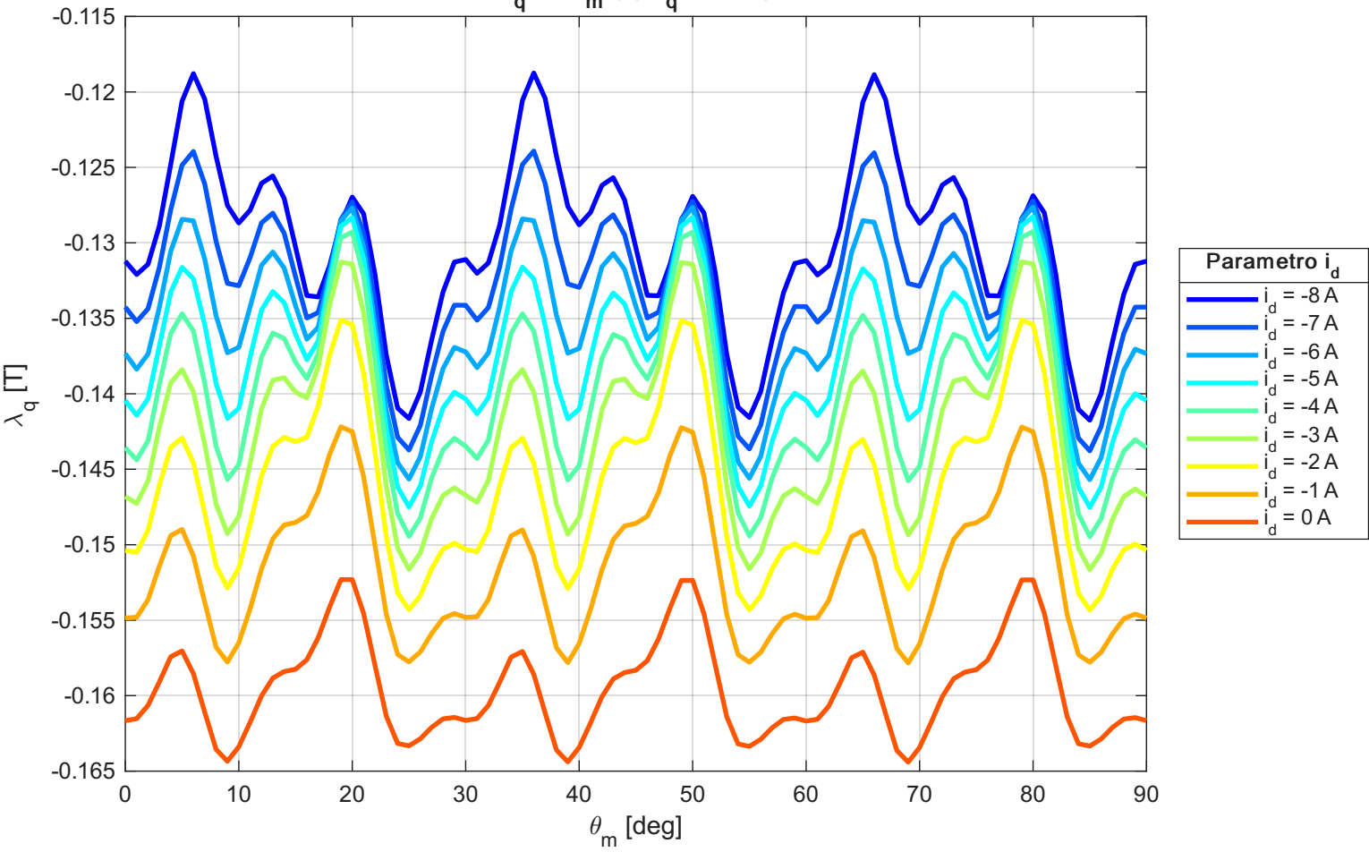
\lambda_q vs \theta_m (@ i_q = -1 A)
