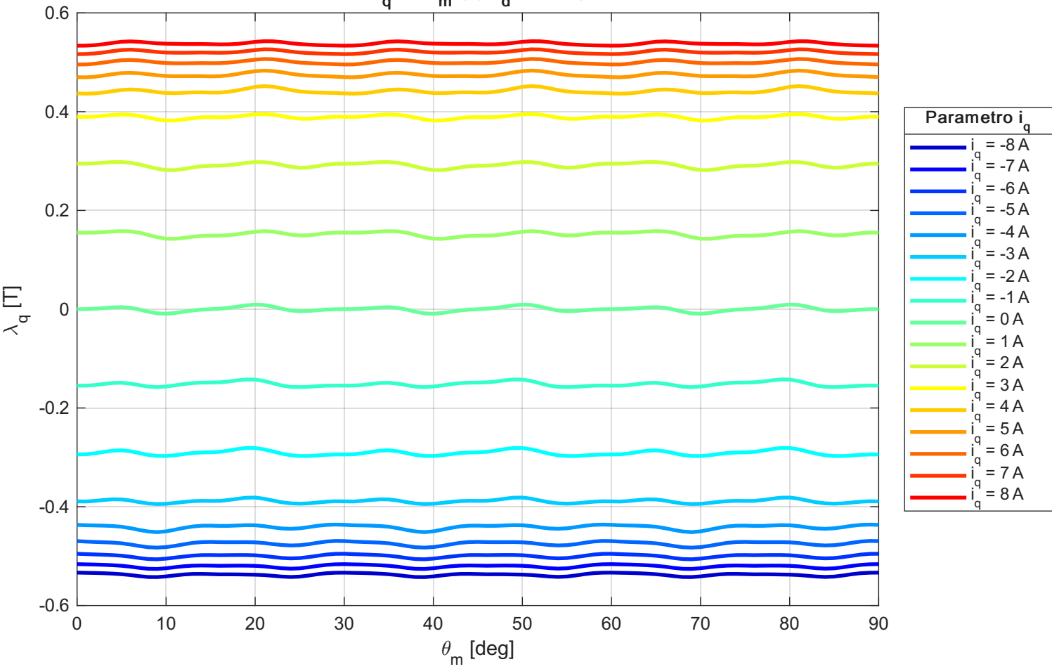
\lambda_q vs \theta_m (@ i_d = -1 A)
