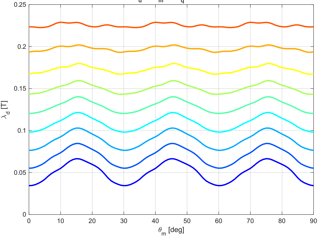
\lambda_d vs \theta_m (@ i_q = 1 A)
