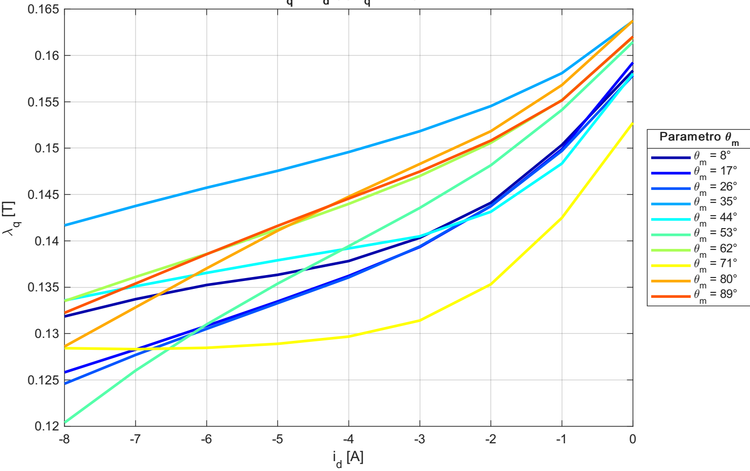
\lambda_q vs i_d (@ i_q = 1 A)
