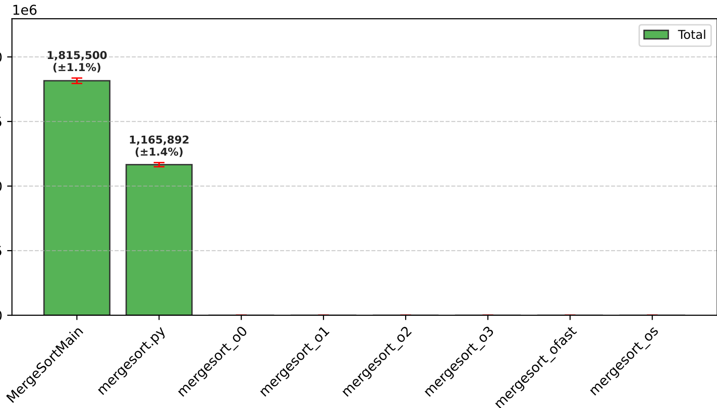
Branches (Total)
