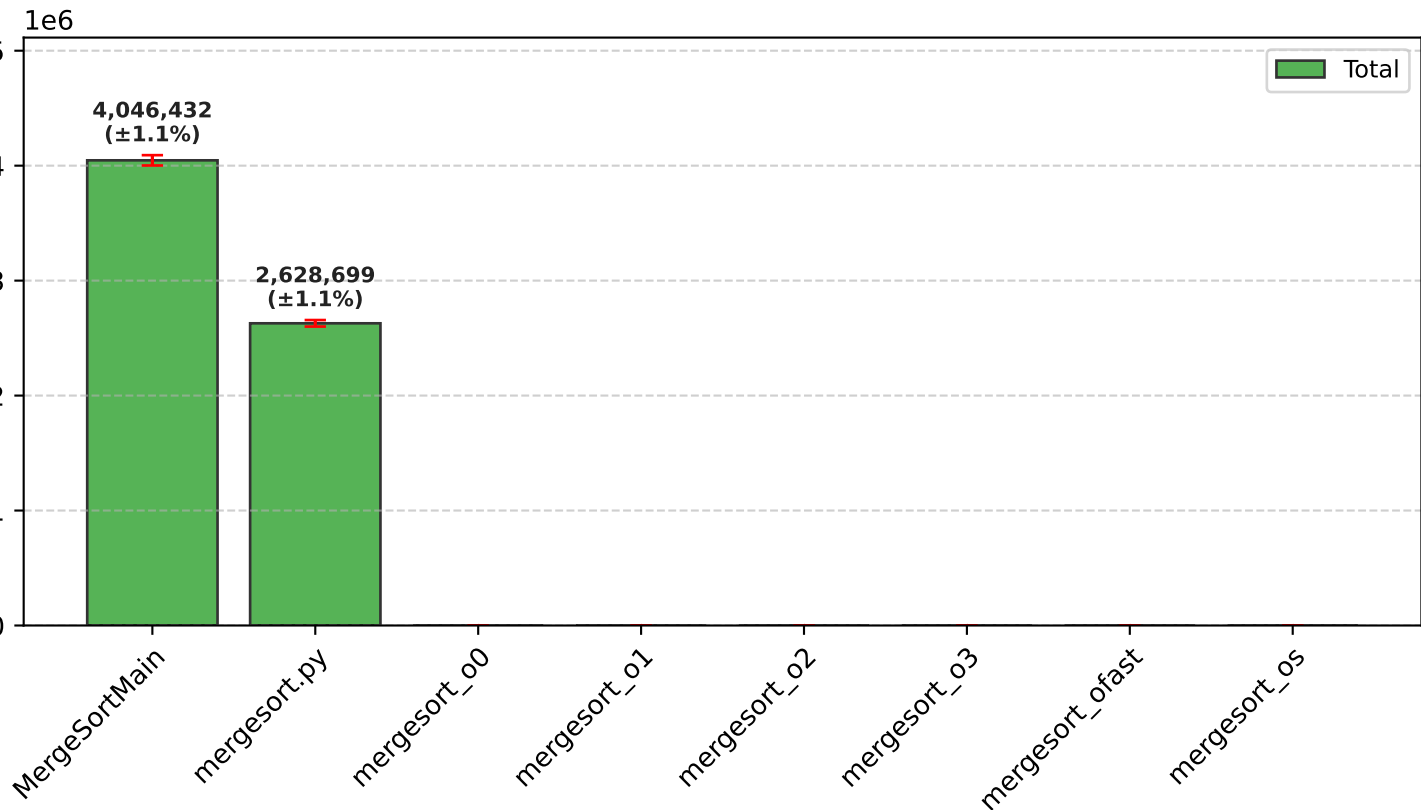
LLC Loads
