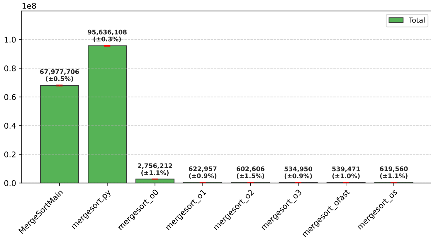
Branch Misses
