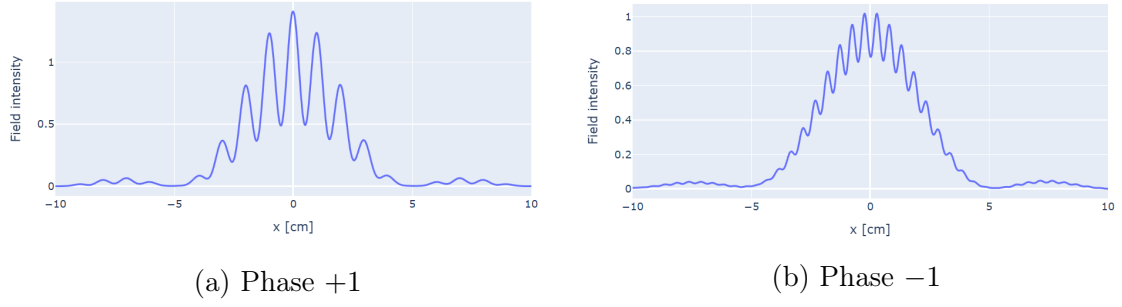
Figure 7: The maxima and the minima swap each time the visibility becomes zero
