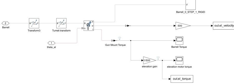
Figure 13: Simulink architecture of the Elevation subsystem.
