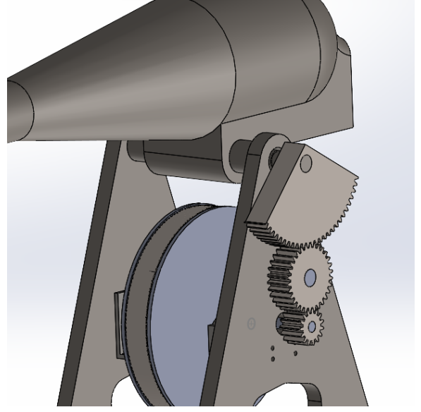
Figure 3: Elevation sector gear, 120^\circ arc, m = 10 , Z_{eq} = 75 .
