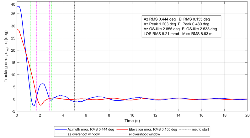
(c) Joint position tracking error
