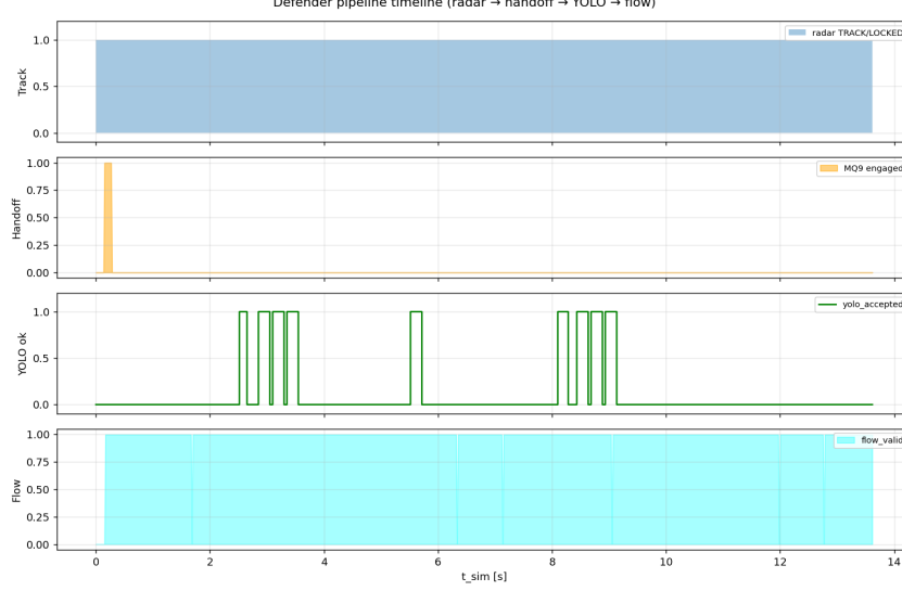
Figure 30: Defender pipeline timeline for log: radar track, MQ-9 handoff, YOLO acceptance, and optical-flow validity.
