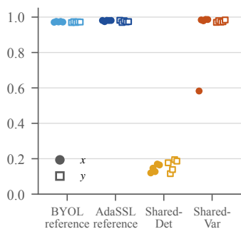
(c) Forecast readout velocity R^2
