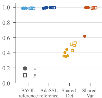
(b) Source projector velocity R^2
