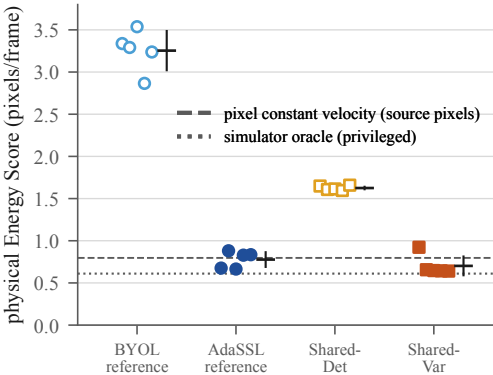
(a) Moving-MNIST
