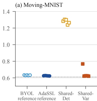
ES of decoded real futures
