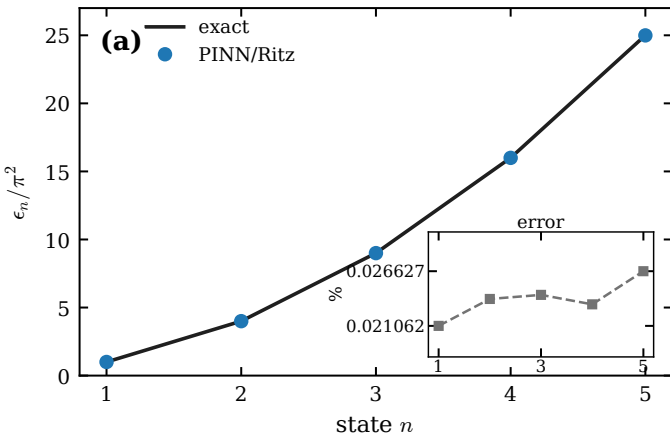
disk doublet
