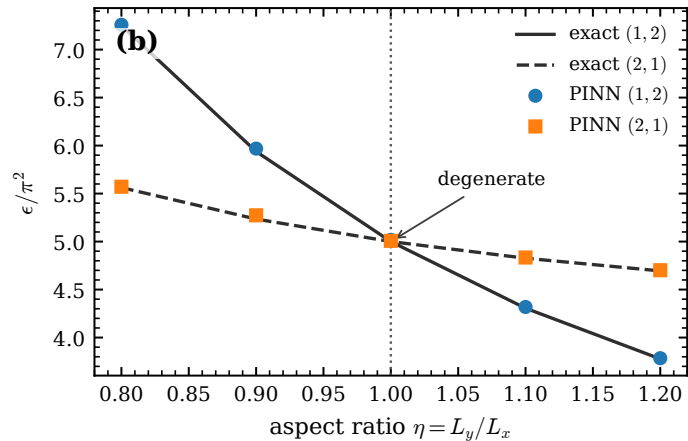
ellipse splitting
