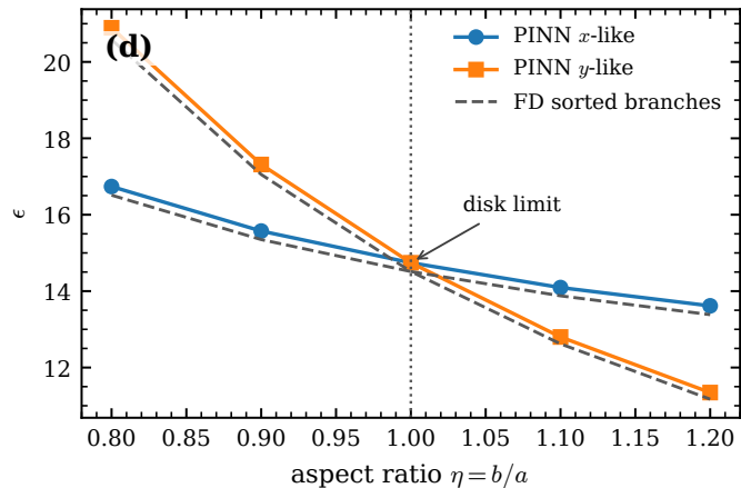
ellipse splitting
