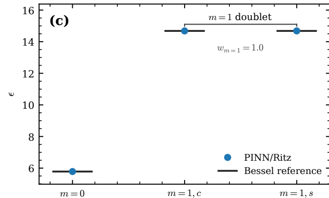
disk doublet
