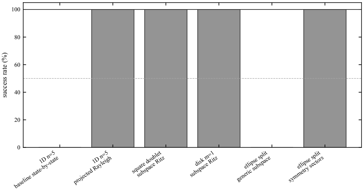
Native-script failure-mode ablation
