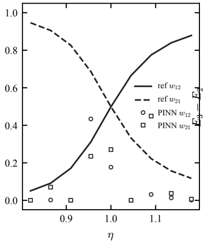
(b) modal exchange
