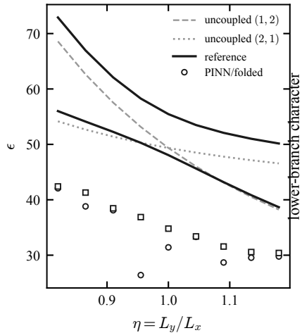
(a) avoided crossing
